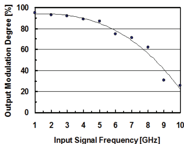
Fig. 23. Output modulation degree versus input signal frequency.
