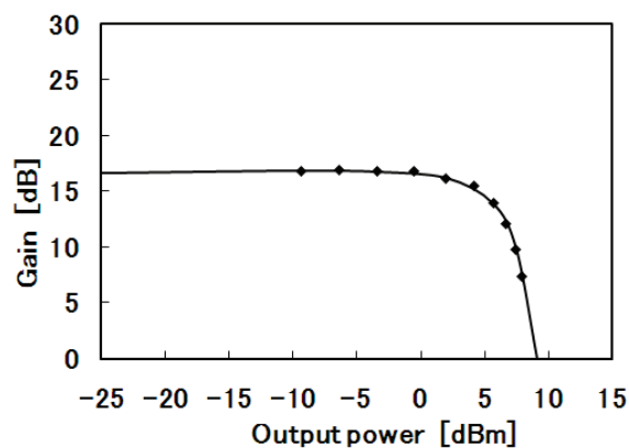
Fig. 11. Characteristic of saturation gain curve for NF-SOA.
