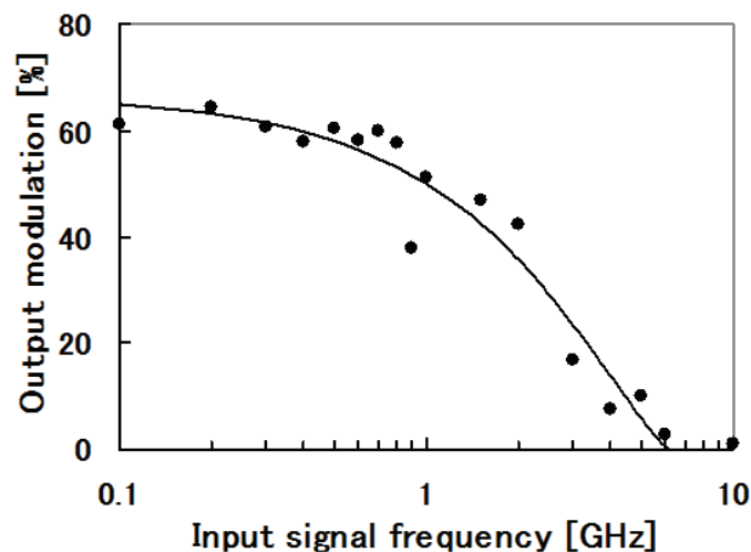
Fig. 19. Output modulation degree versus input signal frequency.
