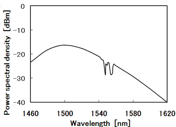
Fig. 12. Amplified spontaneous emission (ASE) spectrum for NF-SOA.
