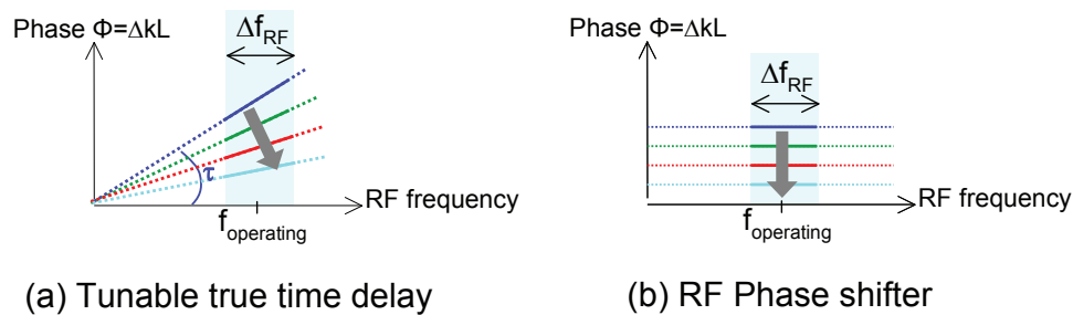
Fig. 2. (a) Illustration of tunable true time delay. (b) Illustration of RF phase shifter.
