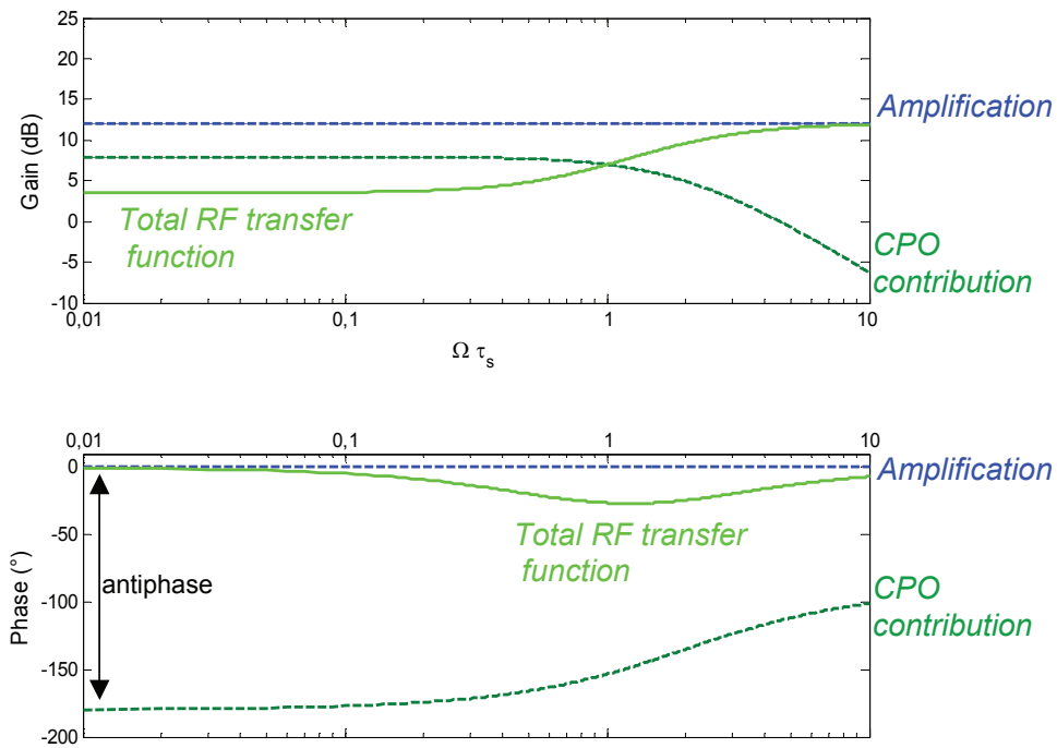
Fig. 5. Contributions and resulting total transfer function.
