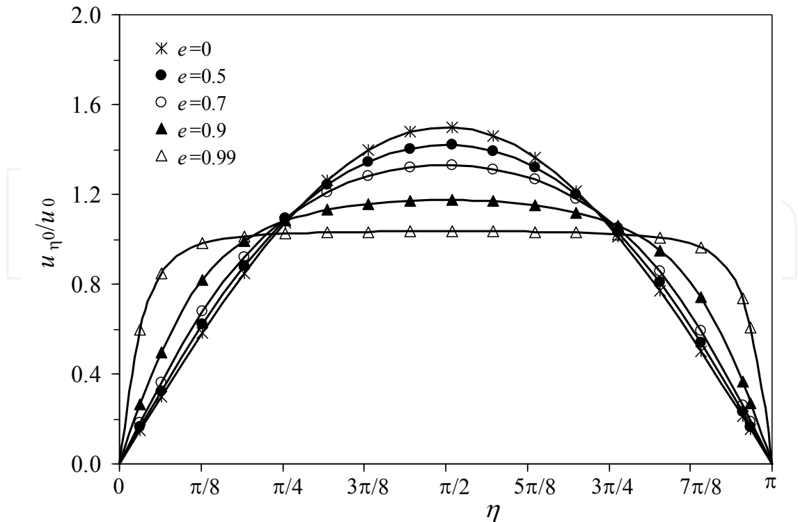
Fig. 2. The dimensionless tangential surface velocity, u_{\eta 0} / u_0 , of a prolate spheroid as a function of \eta , for different values of the eccentricity, e .
