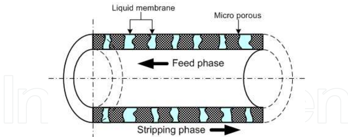
Fig. 2. The microporous hollow fiber liquid membrane
