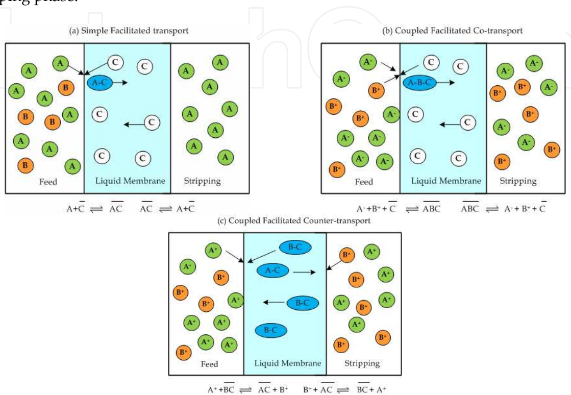
Fig. 3. Schematic pictures of liquid membrane systems (adopted from Bringas et al., 2009)
