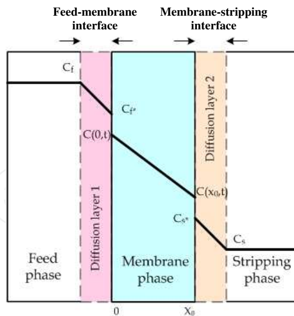
Fig. 5. The proposed steps in Huang’s diffusion model
