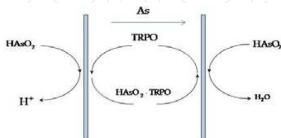
Fig. 9. Schematic representation of neutral As(III) with Cyanex 923
