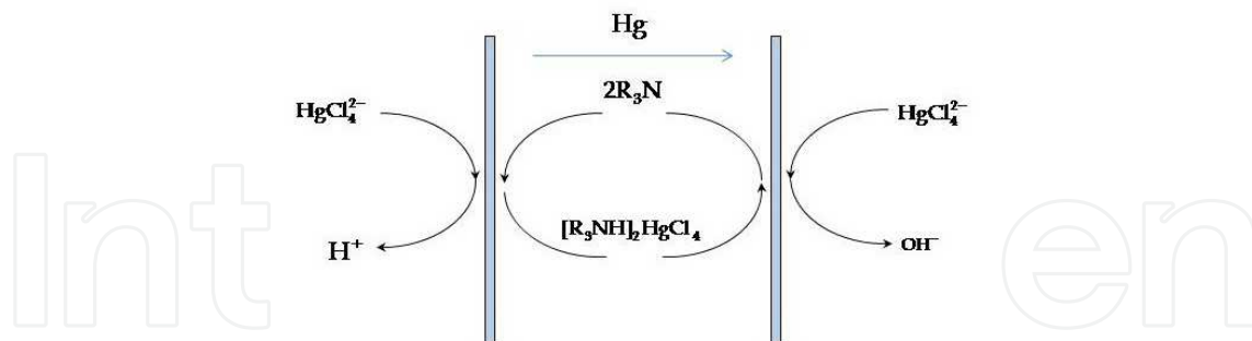
Fig. 10. Co-transport scheme of \text{HgCl}_4^{2-} by TOA extractant
