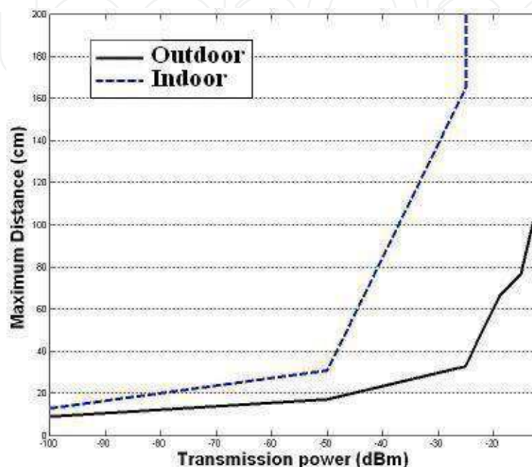
Fig. 11. Minimum Power Required for Communication (Pu, 2009).
