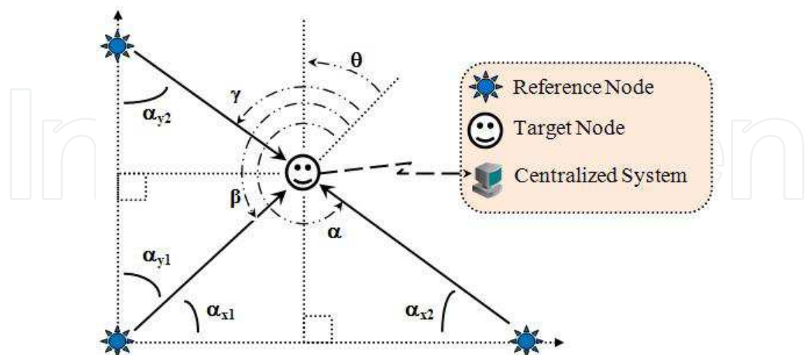
Fig. 6. Estimation in Target Node (Pu, 2009).
