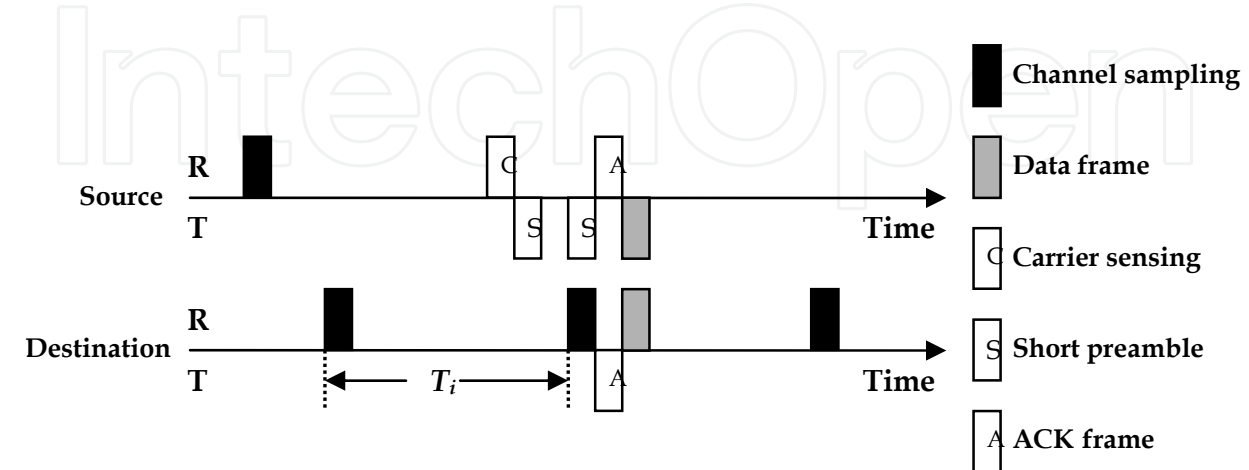
Fig. 9. Basic operation of unsynchronised X-MAC.
