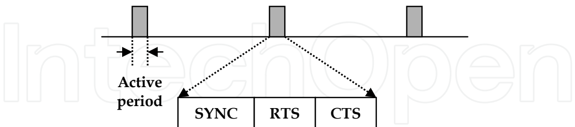
Fig. 4. S-MAC synchronous periodic wake-up scheme.
