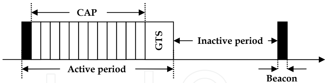
Fig. 6. Superframe structure in beaconed mode IEEE 802.15.4 MAC.
