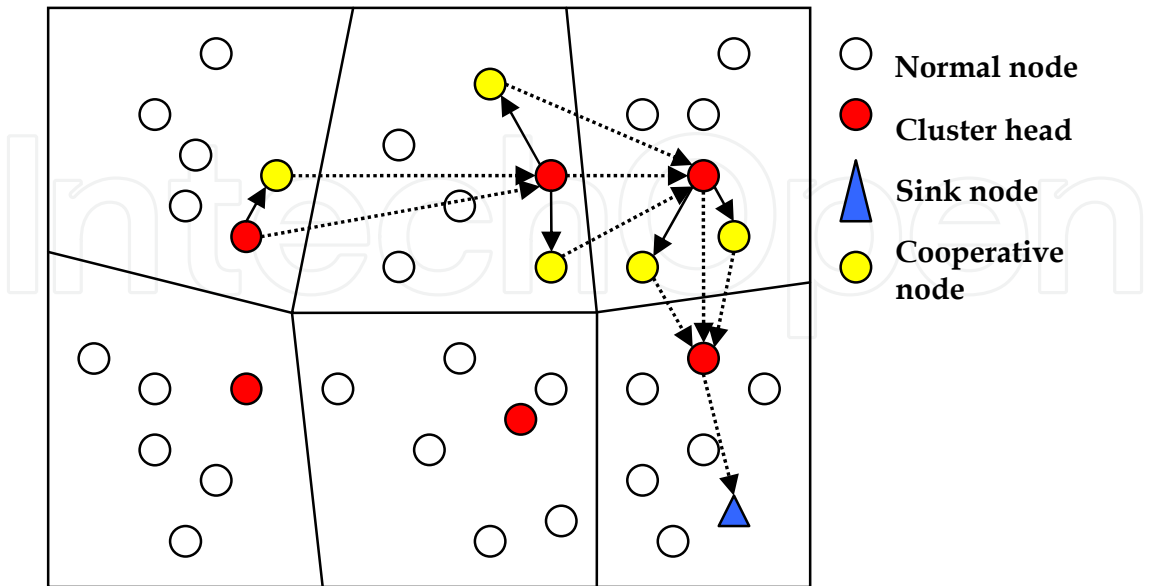
Fig. 10. Multi-hop clustered MIMO-LEACH MAC architecture.
