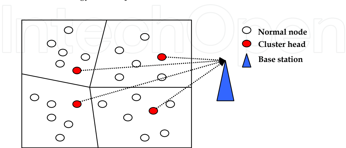
Fig. 3. Clustered LEACH MAC architecture.
