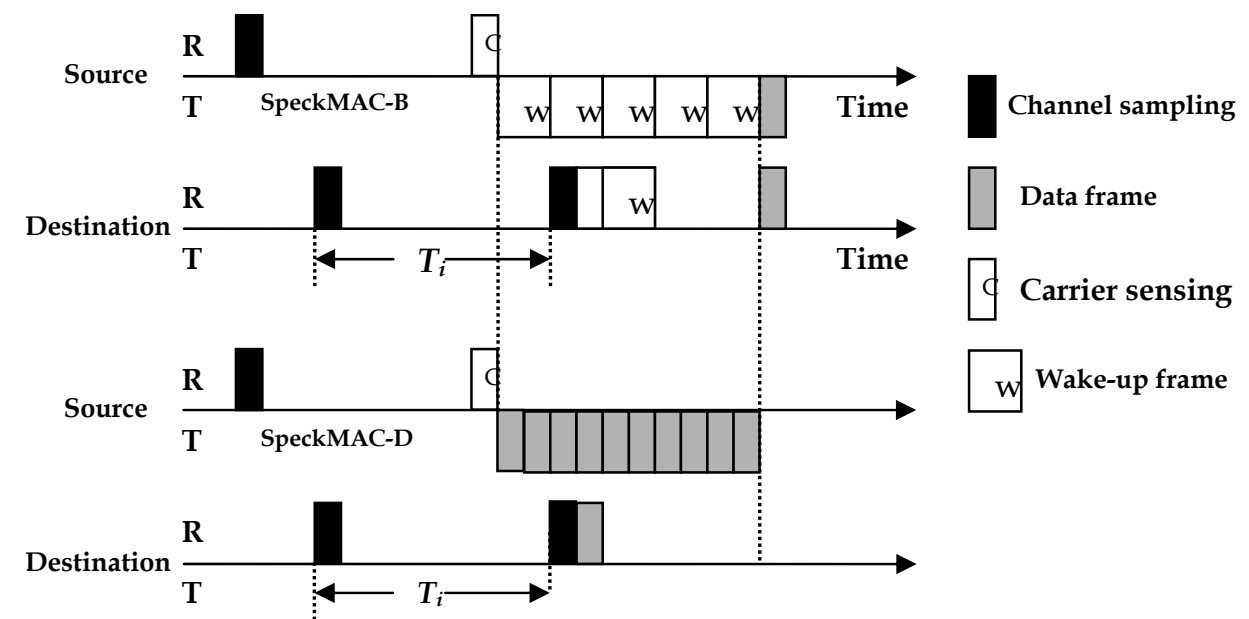
Fig. 8. Basic operation of unsynchronised SpeckMAC.
