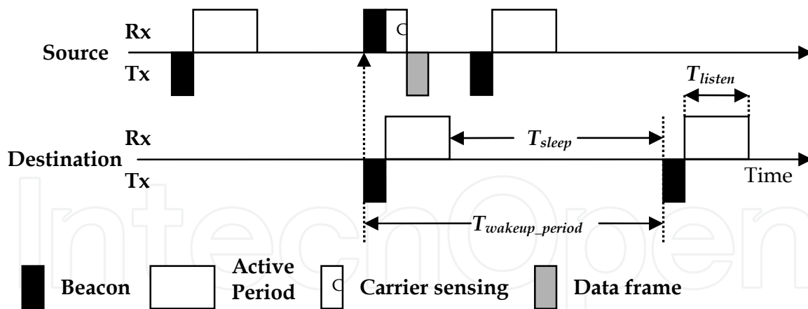
Fig. 2. A synchronous periodic wake-up scheme.
