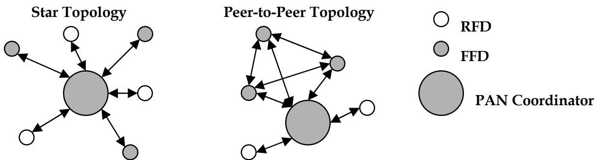
Fig. 5. Topology configurations supported by IEEE 802.15.4 standard.
