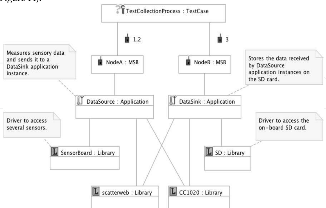
Fig. 14. Test case within an application
