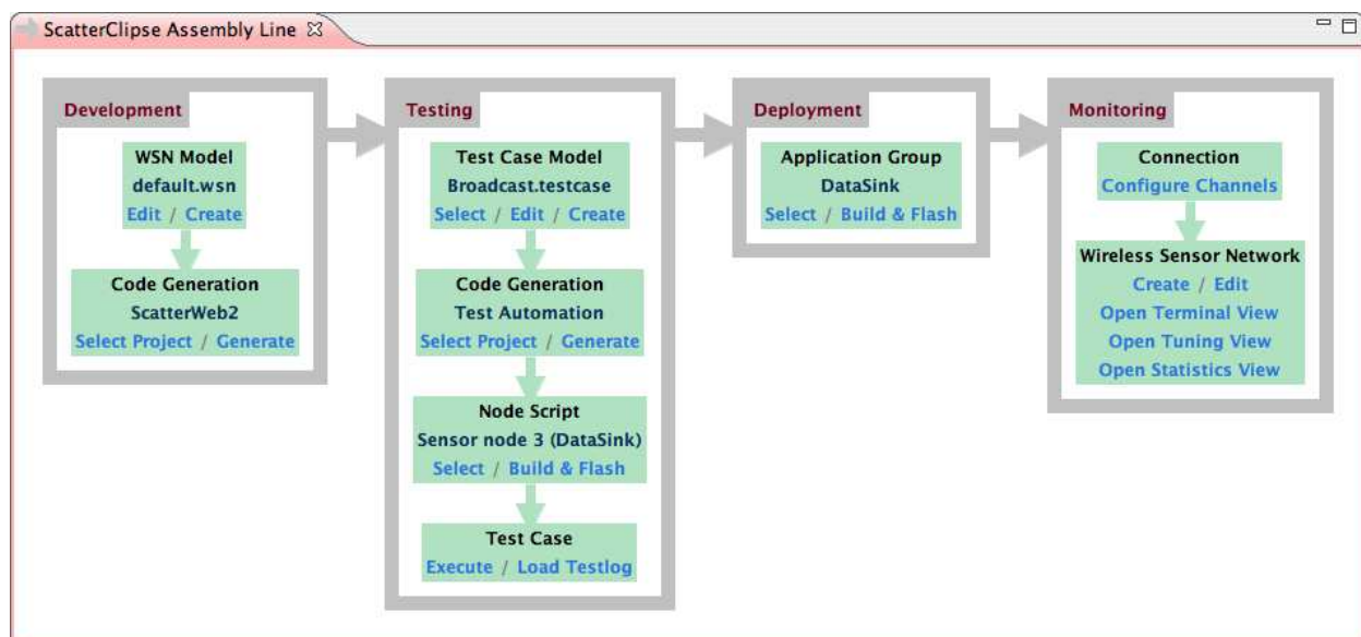
Fig. 20. The Scatterclipse Assembly Line
