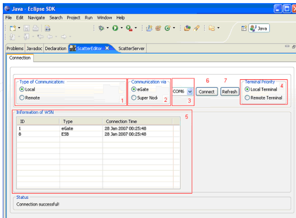
Fig. 15. Connection Tabfolder
