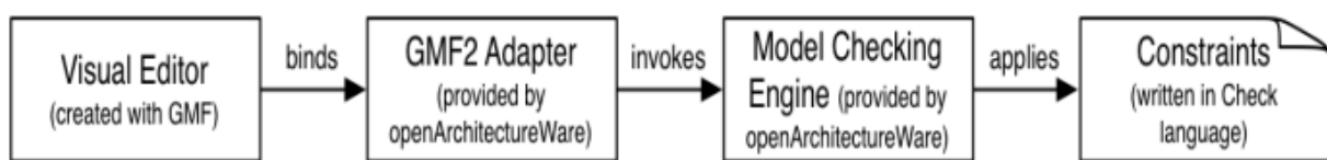
Fig. 10. Live-Validation Components
