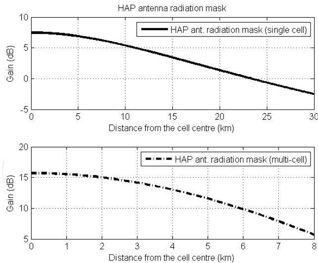
Fig. 4. HAP antenna radiation masks in a single cell and multi-cell formation.
