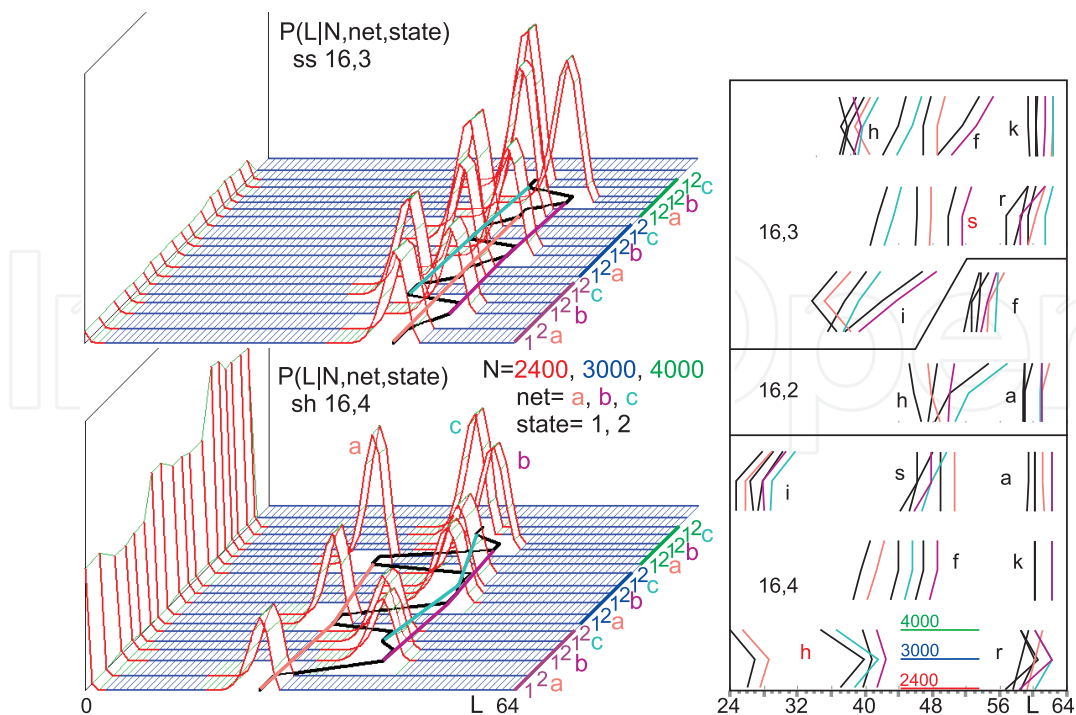
Fig. 8. Individual structure influence on the right peak width. Extreme examples of differences in 3 particular networks ( a, b, c ) on N=2400, 3000, 4000 measured two times, the second time after a random change of all node states, while keeping the structure stable. Value of shift is larger ( s=16 ) than the width of peak which is exactly repeatable (two consecutive cases 1 and 2). The stable character of deviation for a particular network during its three steps of growth is visible, especially in the right diagram. Compare to er which doesn't grow. This diagram contains all the simulated cases depicted only as points of maximum (colour lines) and its standard deviation (black lines).
