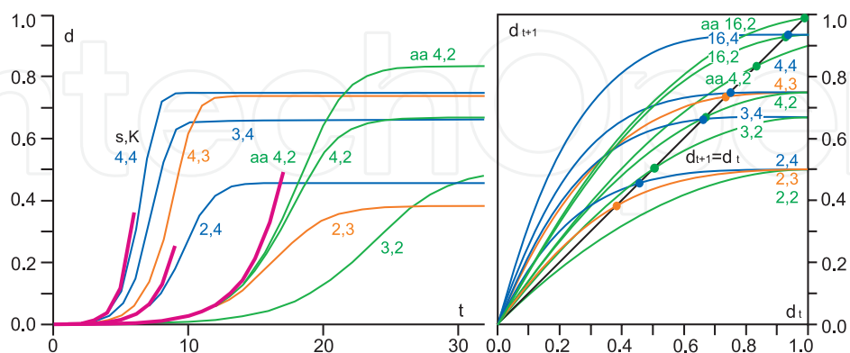
Fig. 5. Theoretical damage spreading calculated using an annealed approximation. On the right - damage change at one time step in synchronous calculation known as the 'Derrida plot', extended for the case s > 2 and for aa network type. The crossing of curves d_{t+1}(d_t, s, K) with line d_{t+1} = d_t shows equilibrium levels dmx up to which damage can grow. Case s, K = 2, 2 has a damage equilibrium level in d = 0 . These levels are reached on the left which shows damage size in time dependency. For s > 2 they are significantly higher than for Boolean networks and for aa than for the Kauffman network. All cases with the same K have the same colour to show s influence. A simplified expectation d(t) = d_0 w^t using coefficient w is shown (three short curves to the left of the longer reaching equilibrium). This approximation is good for the first critical period when d is still small.
