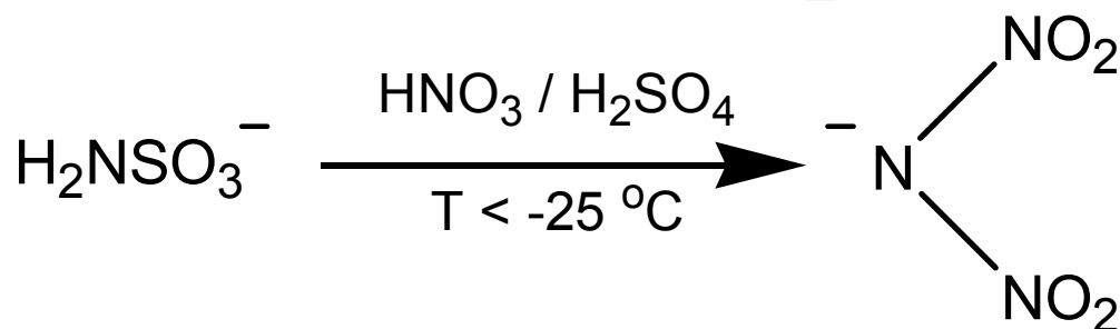
Fig. 4. Synthesis of dinitramide from sulfamic acid.
