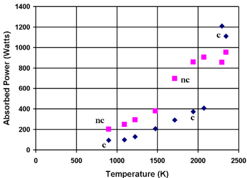
Fig. 3. Power taken by the system (cavity, crucible and mixture) estimated from the forward and reflected power ratio during the test of mixtures of 8 g Compacted (c) and non-compacted (nc) mixtures exposed to 2000 Watts.
