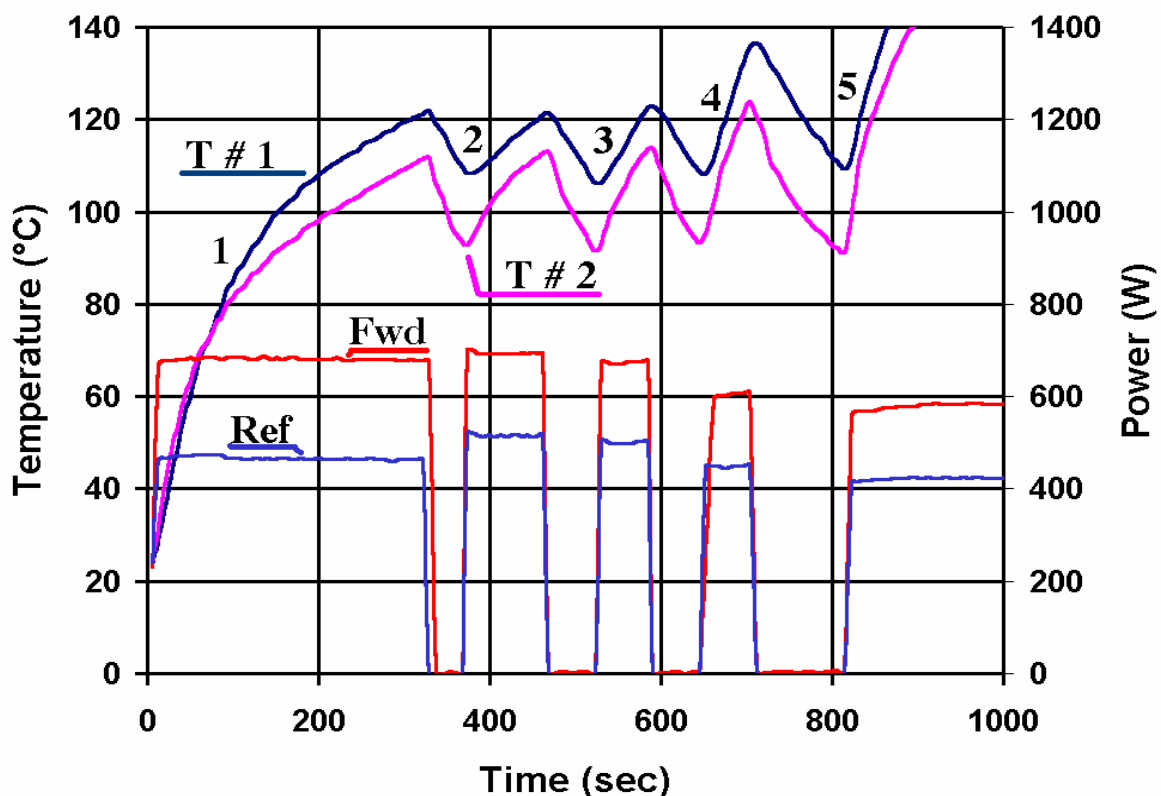
Fig. 8. Temperature measurement of 145 g of alumina, T#1 is one thermocouple located at 3 mm from the centre of the waveguide and T#2 is another one located at 1 mm. Switching of the power supply (points 1-5) shows reliability of thermocouples. Forward and reflected power is also shown.
