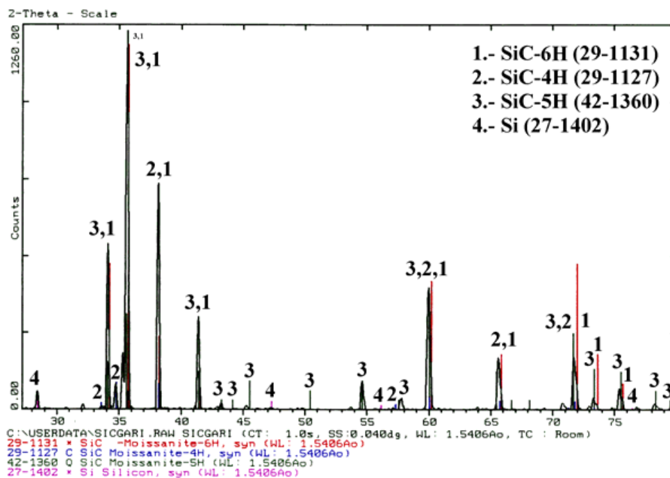
Fig. 5. X-ray diffraction pattern from commercial silicon carbide, notice the mixture of present structures, including silicon. \beta -SiC is not present in this case.
