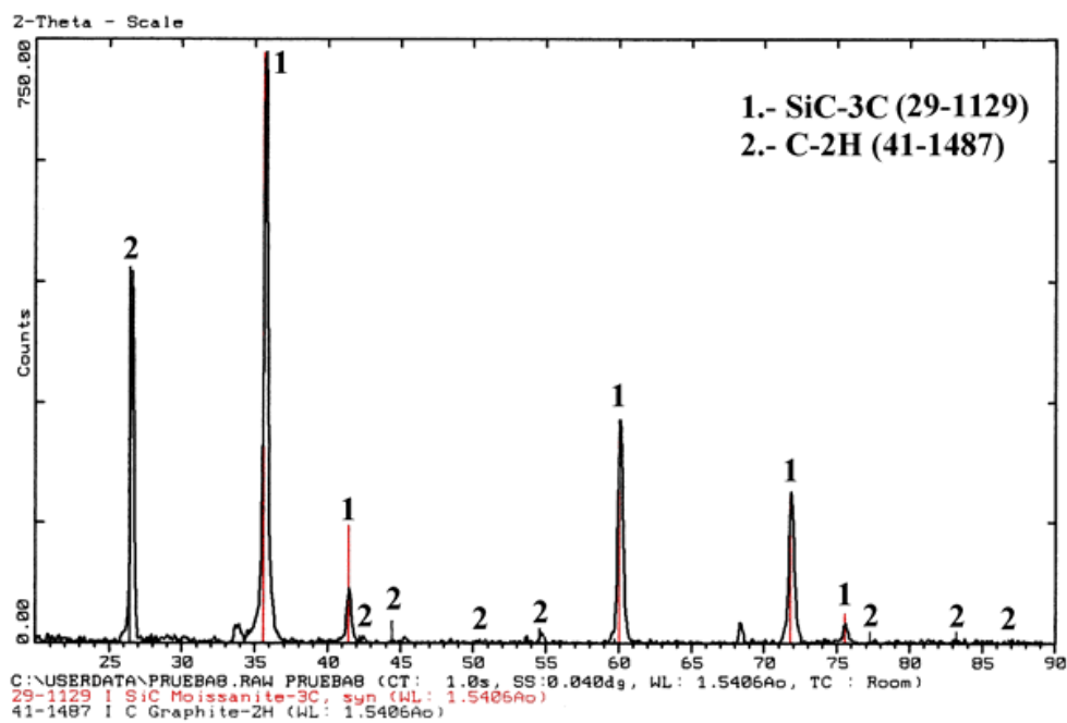
Fig. 4. X-ray diffraction pattern from the black phase in test number 8. The only species found are silicon carbide and graphite. Small unidentified peaks do not form a set for other species, although they might be other silicon carbide polytypes or silicon as element.
