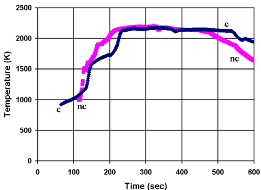
Fig. 1. Comparison between the average thermal evolution of compacted (c) and non-compacted (nc) mixtures of 8 g exposed to 2000 Watts. Temperatures below 900 K were not registered by the optical pyrometer.
