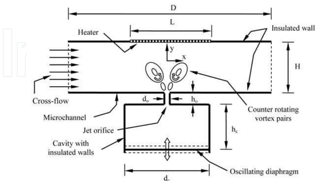
Fig. 4. Schematic diagram of synthetic jet mounted on heat sink in cross-flow configuration
