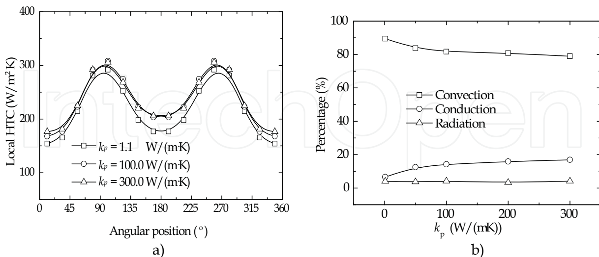
Fig. 14. Effect of k_p on: (a), local HTC; and (b), percentages of different heat fluxes; where u_{exc} = 0.50 m/s (Hou et al., 2010a).
