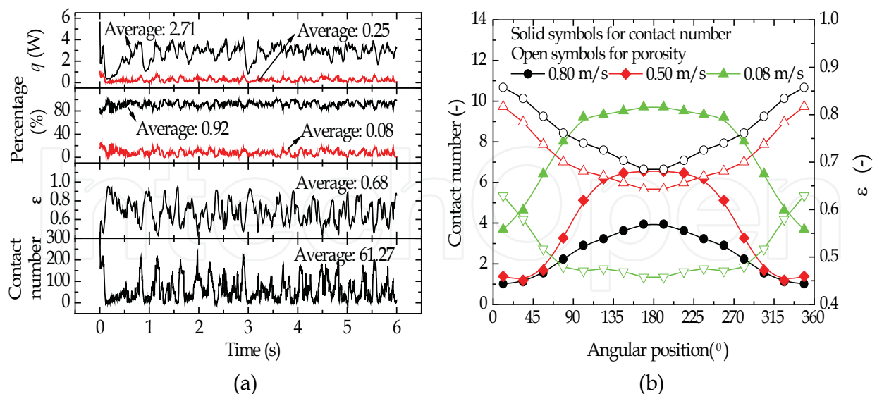
Fig. 13. (a) Overall convective and conductive heat fluxes ( q ) and their percentages ( - , convection; \cdots , conduction), overall contact number (CN) and overall porosity ( \epsilon ) as a function of time, where u_{exc} = 0.40\text{ m/s} (the overall heat flux and CN are the sum of the corresponding values of each section and the overall porosity are the averaged value of all the sections), and (b) local porosity and CN with different u_{exc} (Hou et al., 2010a).
