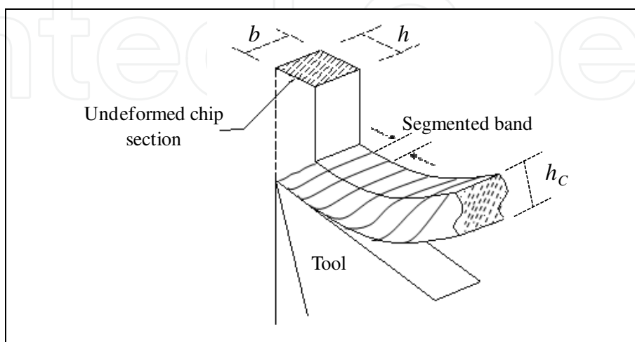
Fig. 8. Orthogonal cutting (uncut chip cross-section)
