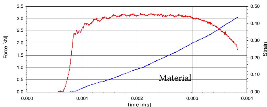
Fig. 9. Load and displacement curve
