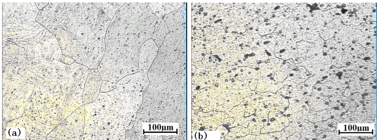
Fig. 5. Microstructure comparison between surface and center area (a) Surface (b) center area
