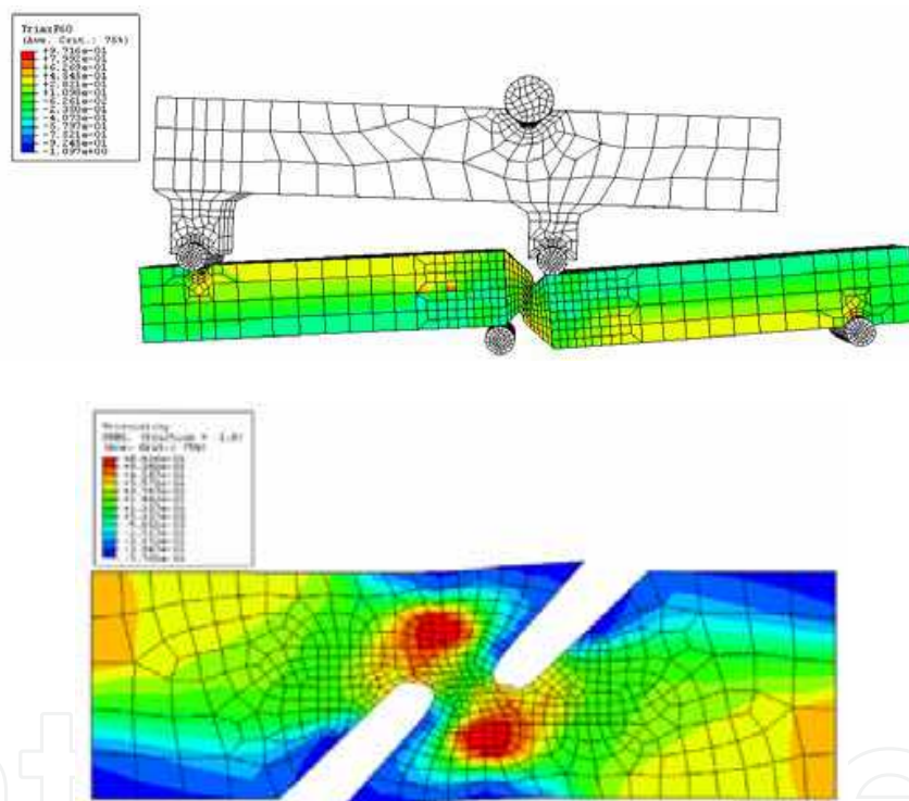
Fig. 18. The distribution of triaxiality for Iosipescu and double notch tensile test
