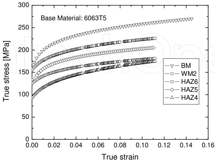
Fig. 24. Uniaxial tensile behavior of different micro zones of joint (6063T5)
