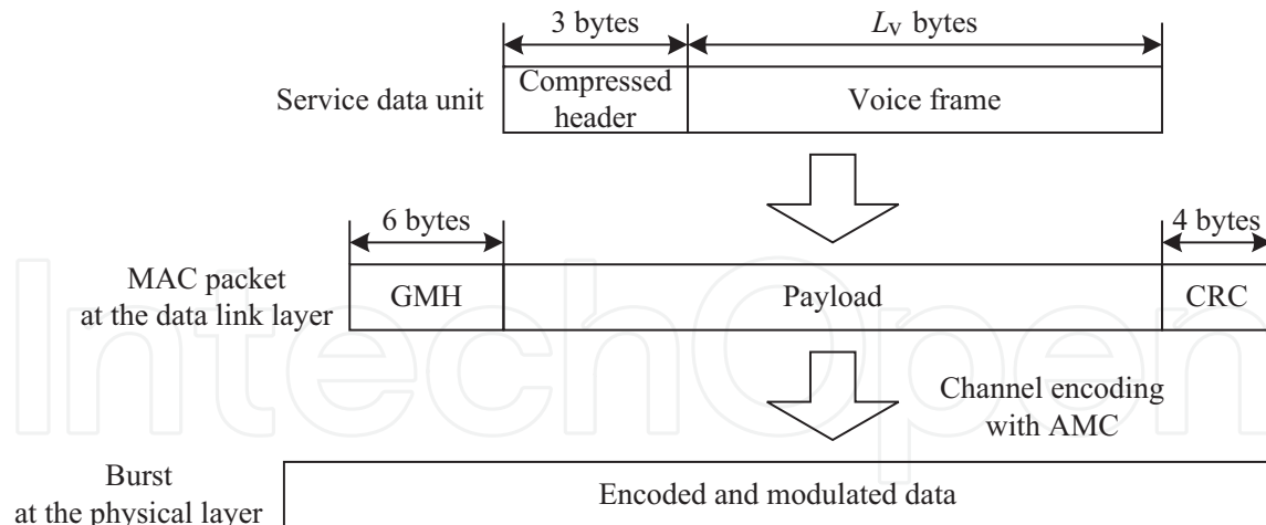
Fig. 2. Packet structure
