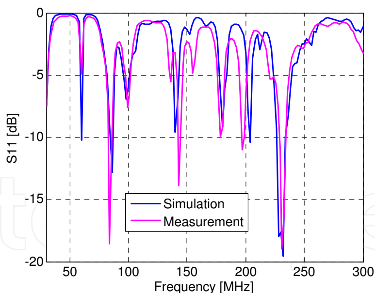
Fig. 12. Comparison of measurement and simulation results for a full car model
