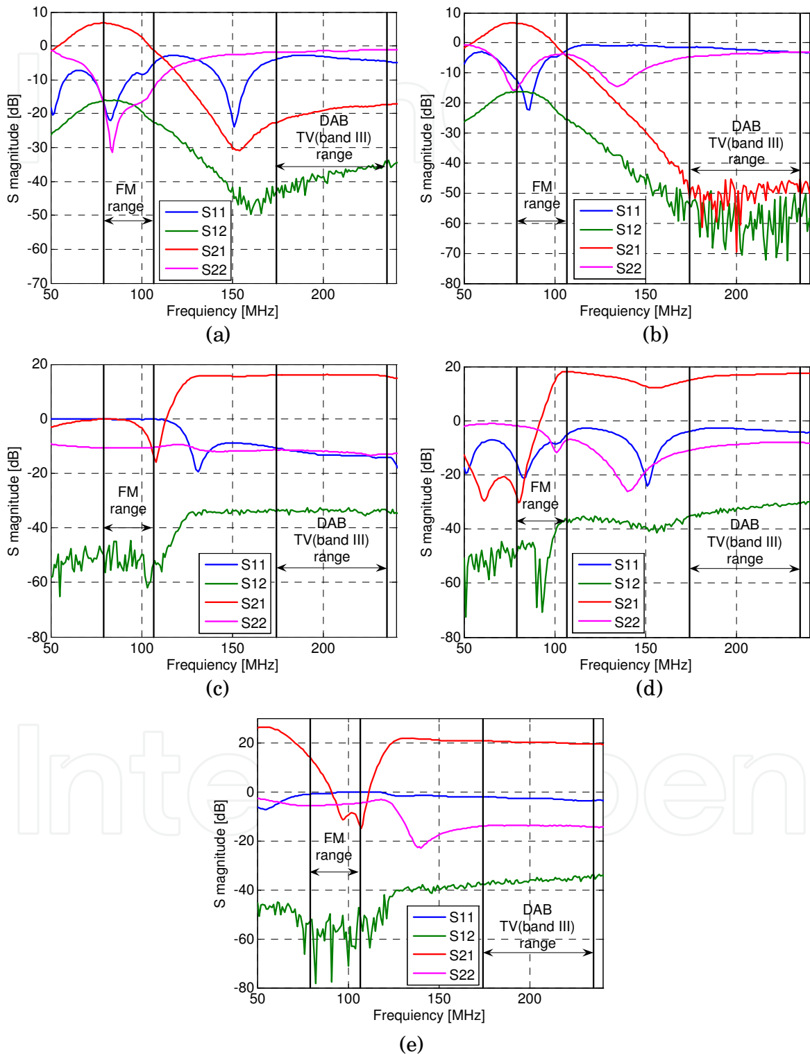
Fig. 25. Measured S-parameters of RF amplifiers as a function of frequency: a) AM/ FM1 amplifier, b) FM2 amplifier, c) DAB amplifier, d) TV1 amplifier, e) TV3 amplifier
