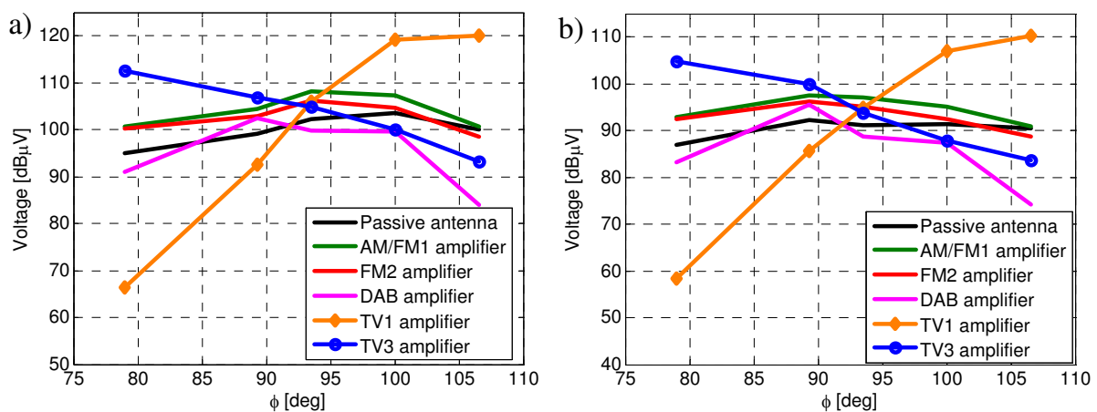
Fig. 29. Averaged received voltage in FM frequency range:
