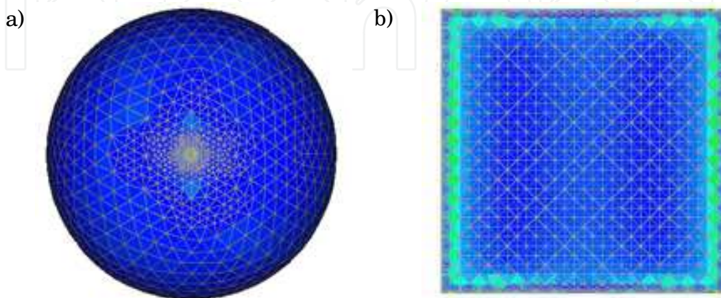
Fig. 3. The adaptive meshes: a) sphere geometry, b) plate geometry
