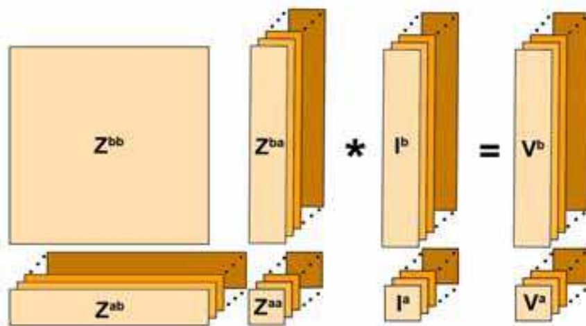
Fig. 13. Structure of multi-partitioned and multi-excitation calculations
