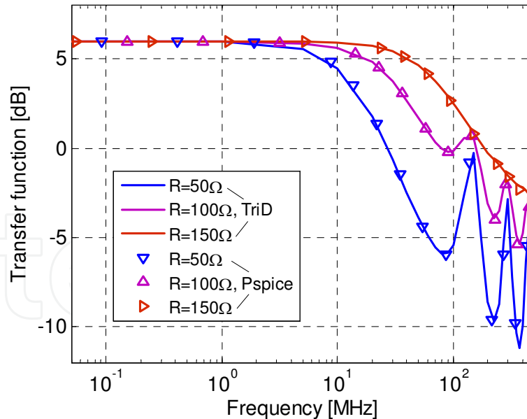
Fig. 7. Comparison of transfer functions calculated by the hybrid MoM (TriD) and PSPICE
