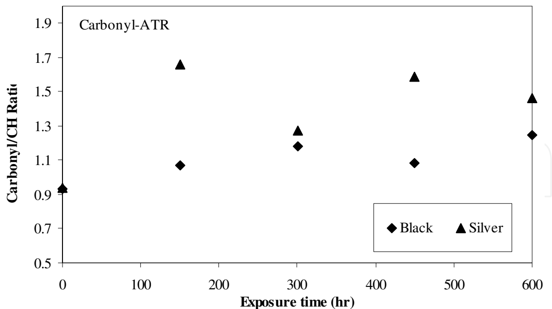
Fig. 9. Normalized absorbances of carbonyl bands of clear coats attached to silver or black basecoats.
