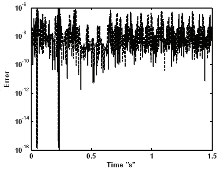
Fig. 4b. Error curve "Duffing case"
