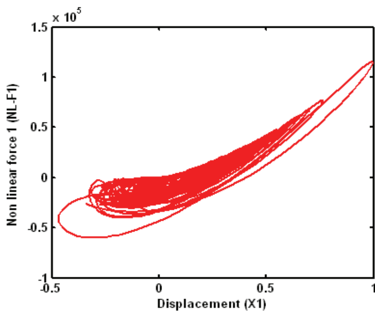
Fig. 21a. Nonlinear forces (X1, NL-F1) "Generalized case: power 1.5 and cubic for weak damping"
