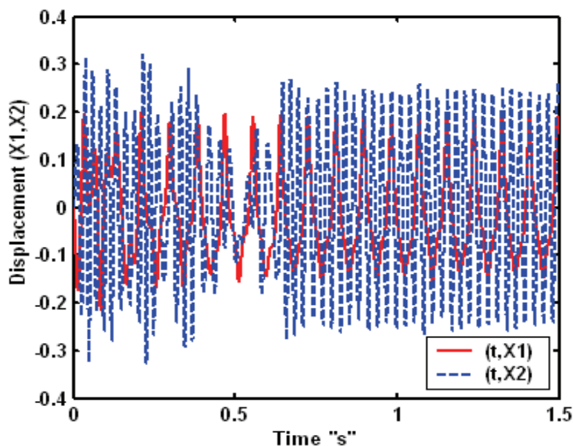
Fig. 2a. Nonlinear temporal responses "Duffing case"
