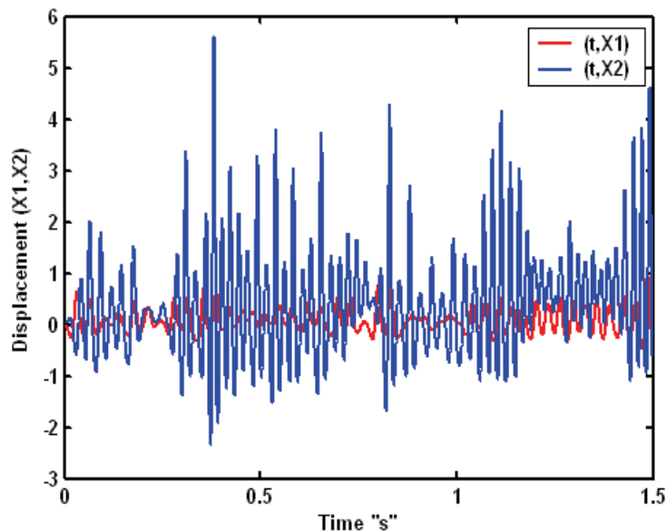
Fig. 19. Temporal nonlinear responses: (X_1(t) and X(t) ) "Generalized case: power 1.5 and cubic for weak damping"
