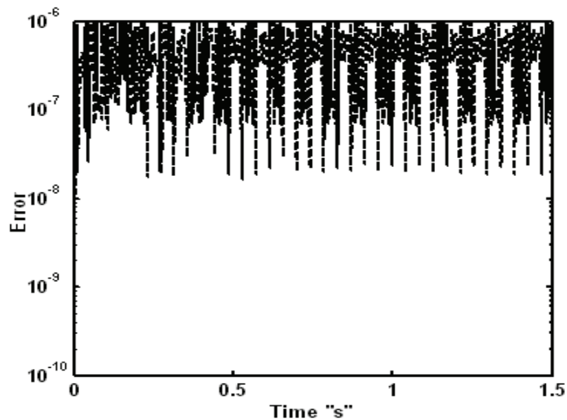
Fig. 7b. Error curve "Van Der Pol case"
