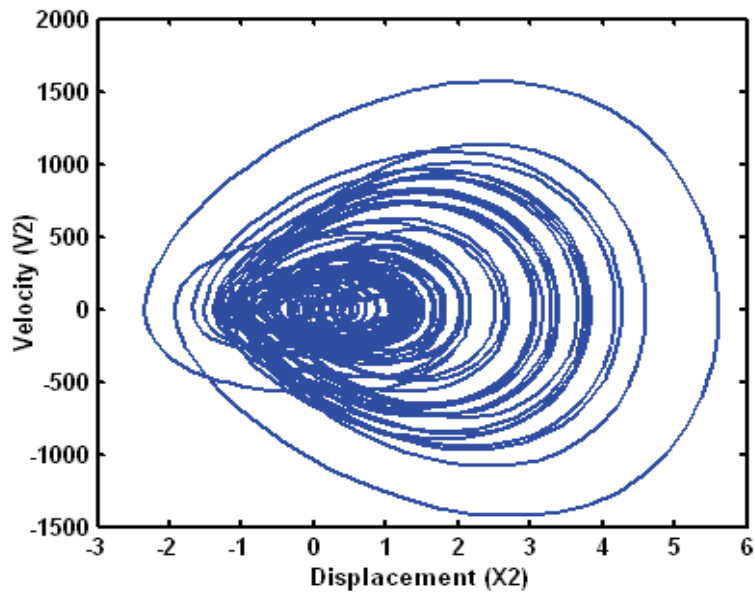
Fig. 20b. Phase diagrams (X2, V2) "Generalized case: power 1.5 and cubic for weak damping"
