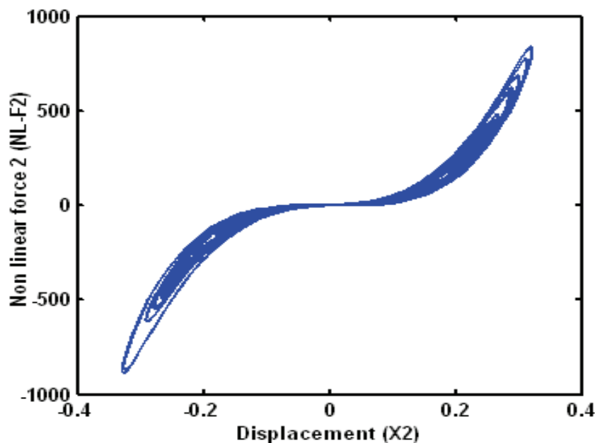
Fig. 3b. Nonlinear forces: (X2, NL-F2) "Duffing case"
