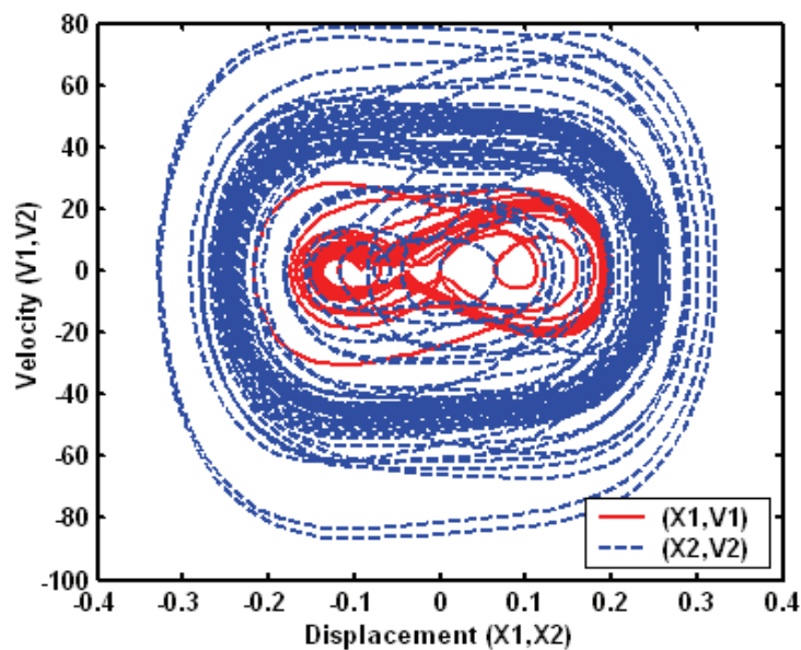
Fig. 2b. Phase diagrams "Duffing case"
