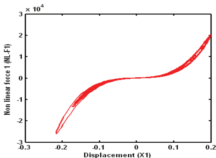
Fig. 3a. Nonlinear forces: (X1, NL-F1) "Duffing case"
