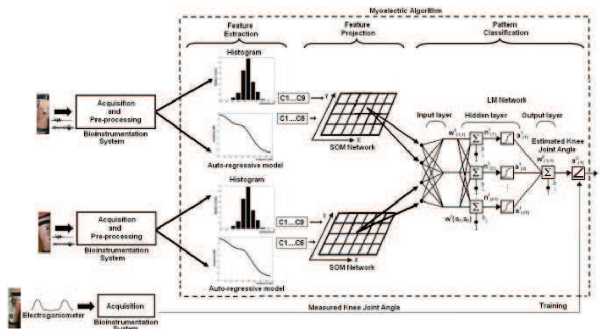
Fig. 4. Block diagram of the proposed knee joint angle estimation algorithm based exclusively on SEMG data.
