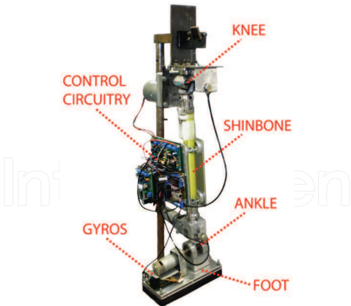
Fig. 1. Prototype of a leg prosthesis for transfemoral amputees.
