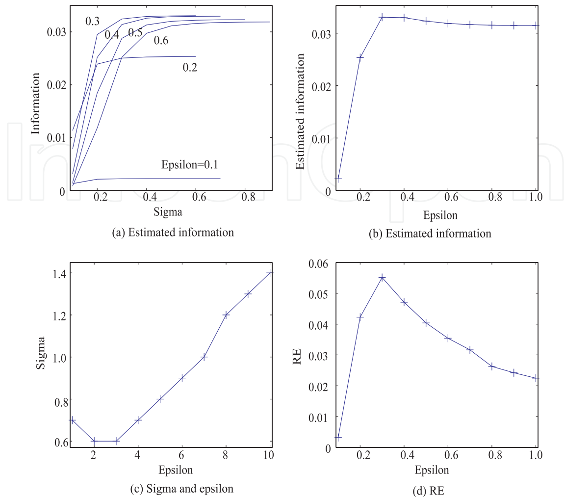
Fig. 24. Information as a function of the parameter \sigma (a) and the parameter \epsilon (b). Optimal values of the parameter \sigma as a function of the parameter \epsilon (c) for the voting attitude problem. The ratio RE as a function of the parameter \epsilon (d).
