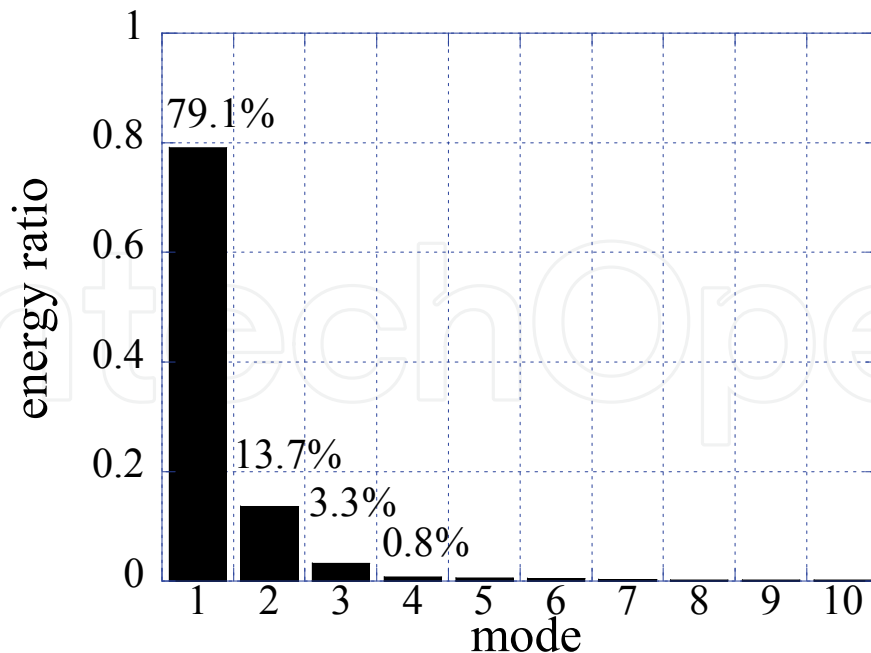
Fig. 13. Energy ratio of the top 10 principal modes of the pressure field distribution.
