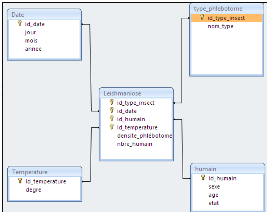
Fig. 5. The model data warehouse diagram
