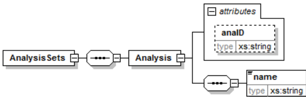
Fig. 4. Structure of the ANALYSIS element
