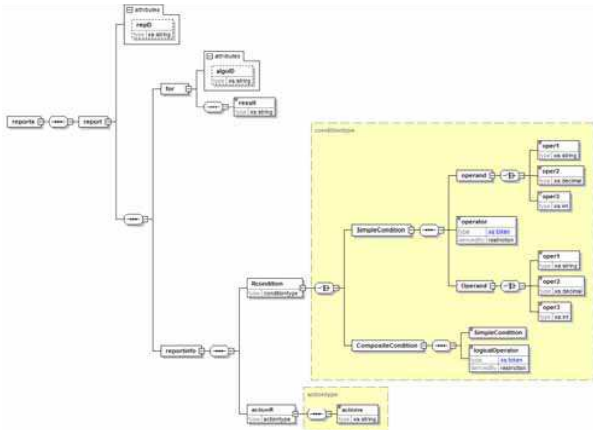
Fig. 7. Structure of the REPORT element
