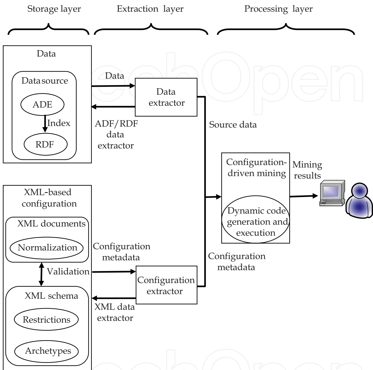
Fig. 1. Framework architecture
