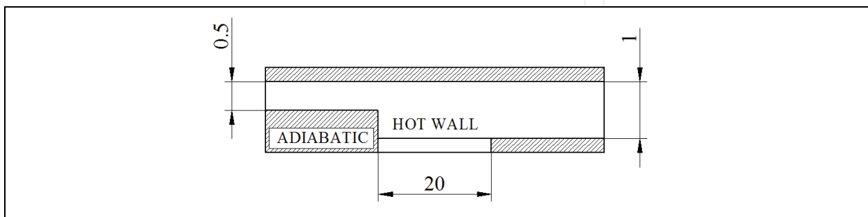
Fig. 1. Dimensionless definition of the 2-D backwards facing step (not at scale). The outlet height of this device is L=450 \mu\text{m} . It works with ideal water ( k=0.598 \text{ W K}^{-1}\text{m}^{-1} , \mu=10^{-3} \text{ Pa s} , c=4180 \text{ J kg}^{-1}\text{K}^{-1} and \rho=998 \text{ kg m}^{-3} ) in an operational point identified by \text{Nu}=5.18 and \text{Re}=100 . These values give the following non-dimensional characterization of the stationary heat flow: \chi=0.074 , \eta(\bar{T}_H)=0.071 , \theta(\bar{T}_p)=0.96 , Z=26 and Y=0.34 .
