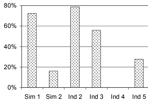
Fig. 11. Average fractions of false predictions obtained from CTs for consistent data subsets (including single records)
