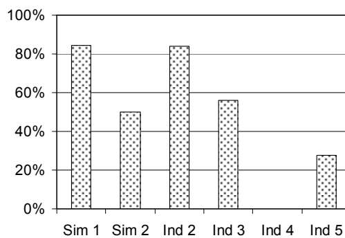
Fig. 15. Fractions of CTs rules with redundant conditions
