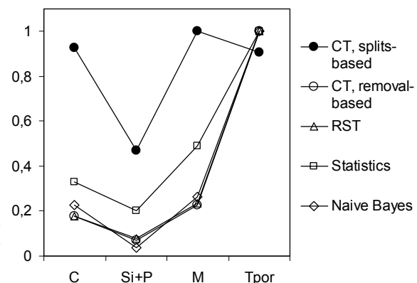
Fig. 10. Relative significances of input variables, obtained by various methods for two industrial data sets related to the feeding of grey cast iron castings: Ind 4 – requirement of feeder application assumed as the output (2 categories), Ind 5 – requirement and size of feeder assumed as the output (3 classes)
