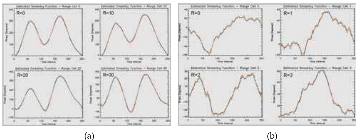
Fig. 12. (a) Demodulation sequences for every 10 th range cell for the case of an internal gravity wave; (b) demodulation sequences for adjacent range cells during a transient event of unknown origin. Data obtained with the Jindalee radar
