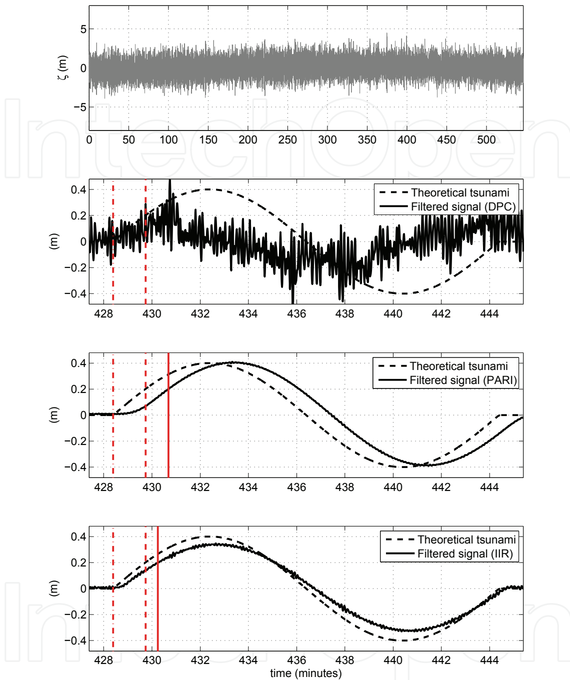
Fig. 10. Upper panel: analyzed sea-level record (resulting from the superposition of Venice tide, a wind-wave signal characterized by a significant height H_{m0}=4.0 m, peak period T_p=8.0 s and a sinusoidal tsunami of amplitude a=0.4 m and period T=16.0 minutes). Lower panels: comparison between the filtered signals resulting from the application of DPC, PARI and IIR-TDF algorithm, and the theoretical sine-like tsunami. Vertical dot-dashed and dashed lines represent the instants at which the sine-like tsunami starts and exceeds the selected threshold respectively ( TS_{amp}=0.2 m). Vertical continuous line represents the instants at which the filtered signal exceeds the same threshold.
