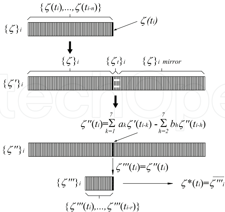
Fig. 4. Proposed algorithm scheme: wind-wave filtering part.
