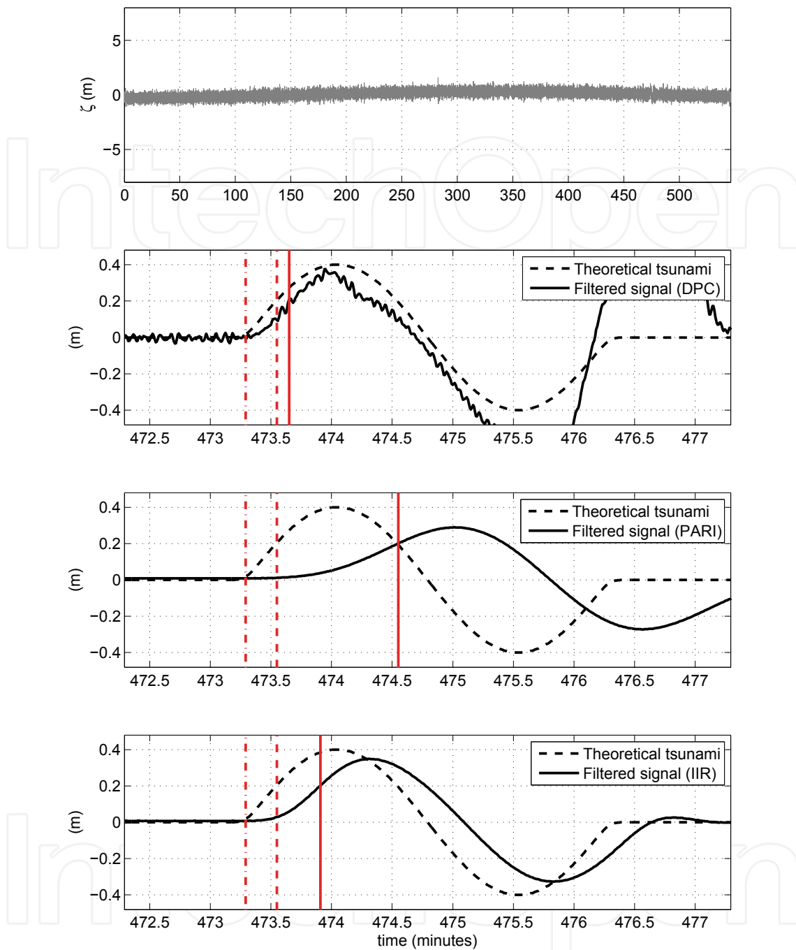
Fig. 8. Upper panel: analyzed sea-level record (resulting from the superposition of Venice tide, a wind-wave signal characterized by a significant height H_{m0}=1.0 m and a peak period T_p=4.0 s and a sinusoidal tsunami of amplitude a=0.4 m and period T=3.0 minutes). Lower panels: comparison between the filtered signals resulting from the application of DPC, PARI and IIR-TDF algorithm, and the theoretical sine-like tsunami. Vertical dot-dashed and dashed lines represent the instants at which the sine-like tsunami starts and exceeds the selected threshold respectively ( TS_{amp}=0.2 m). Vertical continuous line represents the instants at which the filtered signal exceeds the same threshold.
