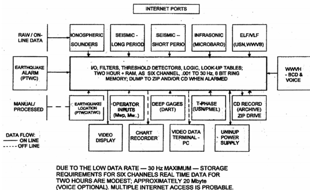
Fig. 4. Data flow, Tsunami genesis experiment laboratory.
