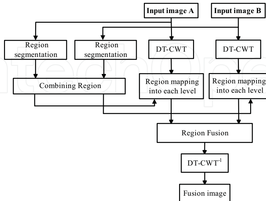
Fig. 1. Diagram of the proposed region-based method with DT-CWT
