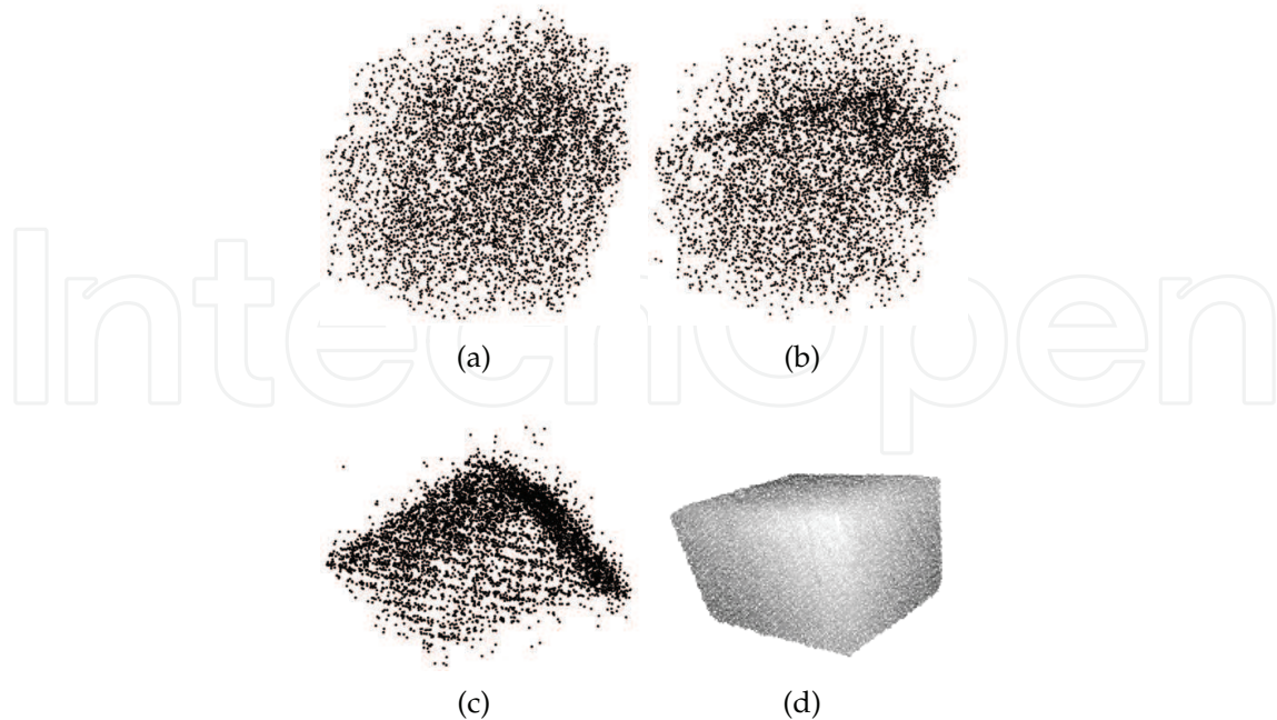
Fig. 19. Cube disparity map. a) Initial (random) configuration. b) After 500 iterations. c) After 5000 iterations. Three faces of the cube are clearly visible. d) After 10000 iterations.
