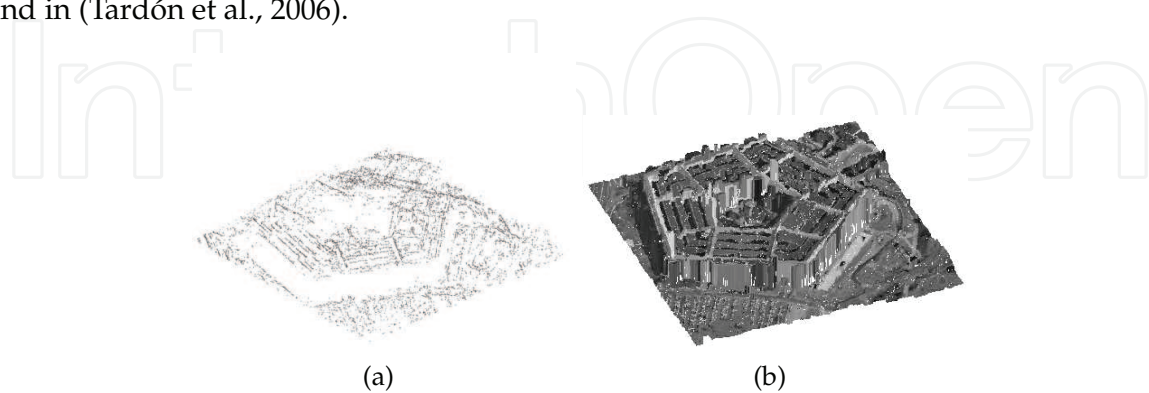
Fig. 25. Disparity map for the pentagon stereo pair after 5000 iterations of the MRF based stereo correspondence algorithm. a) Matched points. b) 3D reconstruction. Surface interpolated using planar patches (Bradley & Vickers, 1993)
