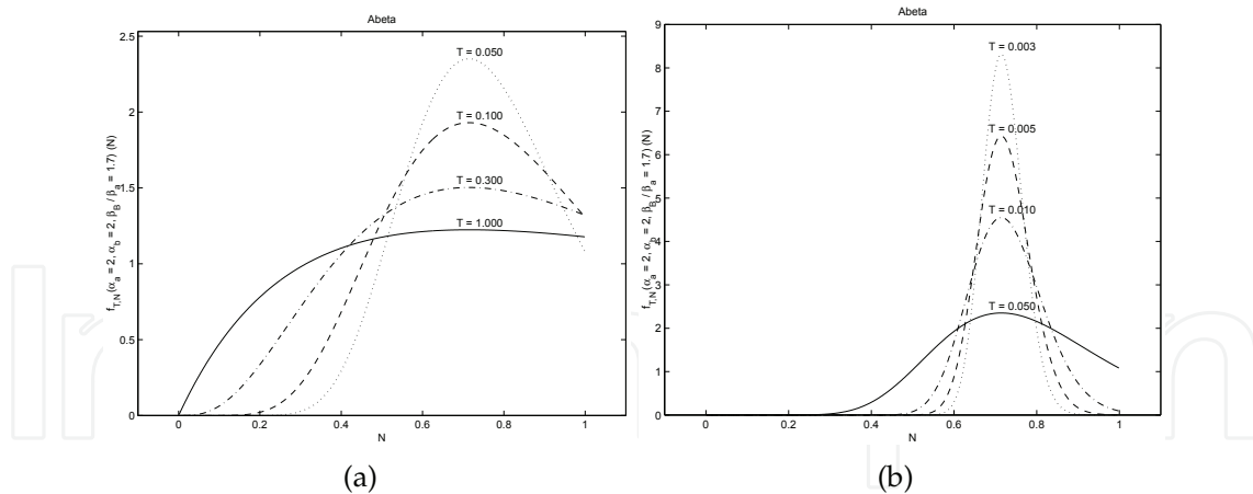
Fig. 8. Exaggeration of the modes of a probability function with decreasing temperature.
