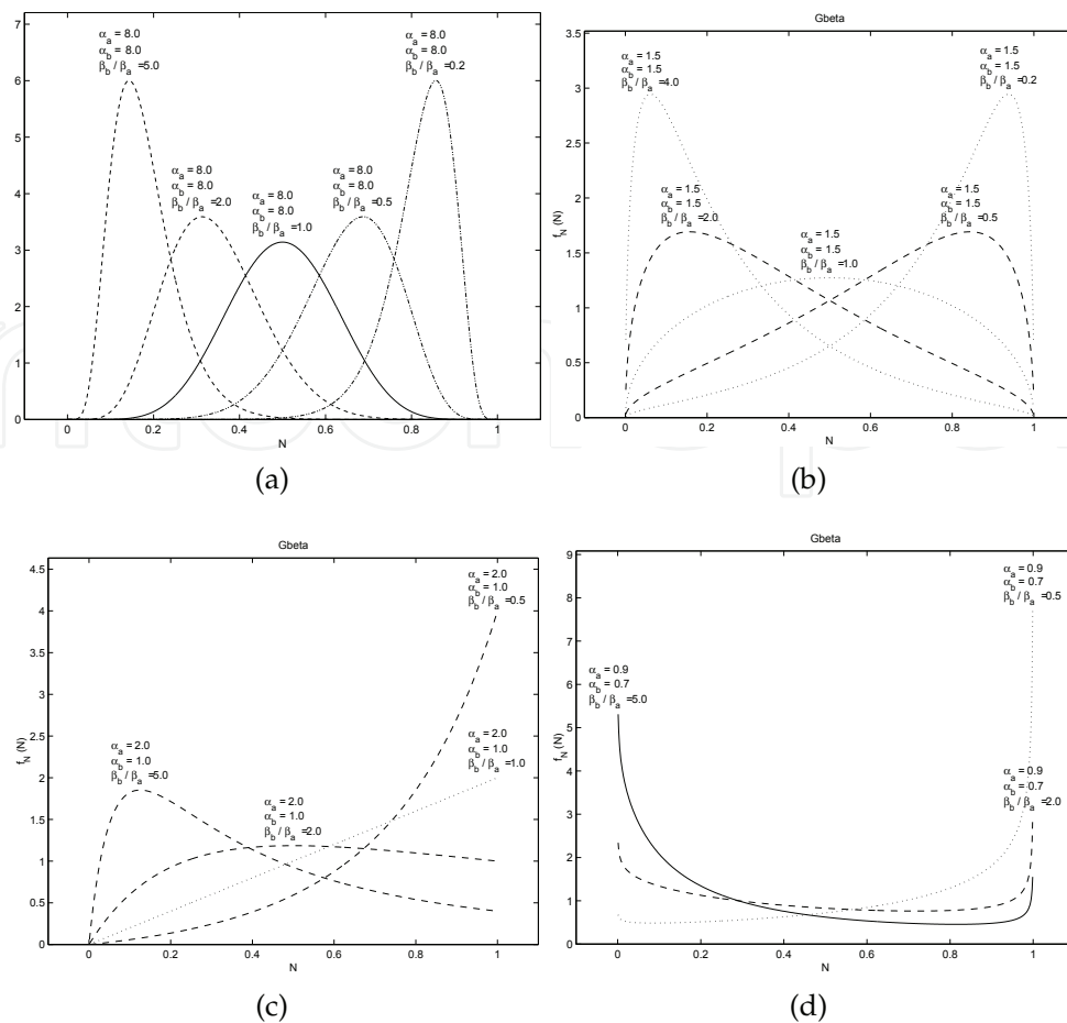
Fig. 15. Gbeta_{\nu, (\alpha_a, \alpha_b, \frac{\beta_b}{\beta_a})}(\nu) .
