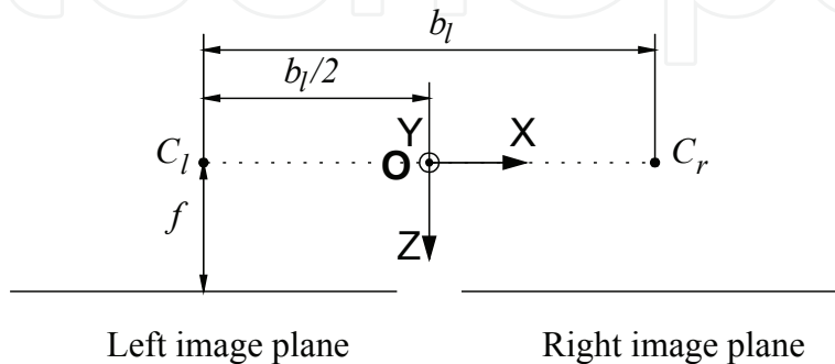
Fig. 12. Stereo system with parallel cameras of small aperture.
