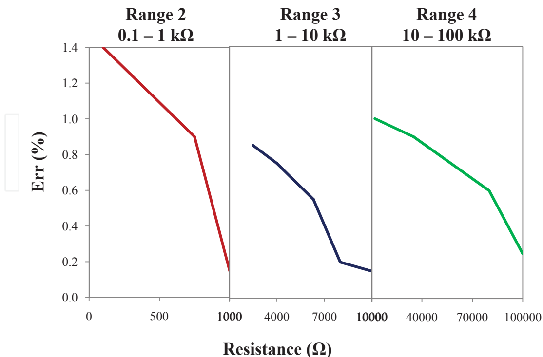
Fig. 5. Home made \mu conductometer. Errors of resistance measurements at three ranges measured by a \mu conductometer.
