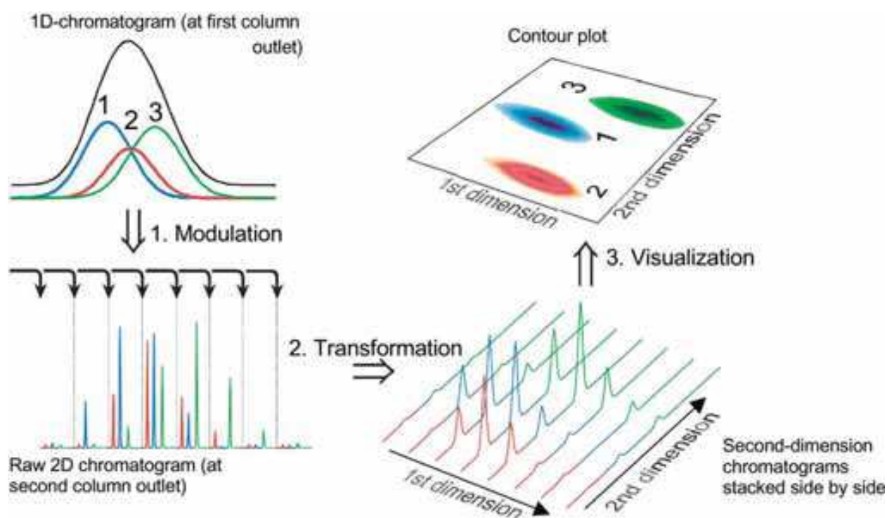
Fig. 6. Generation and visualization of a GC x GC chromatogram (From Dallüge et al., 2002. With permission.).
