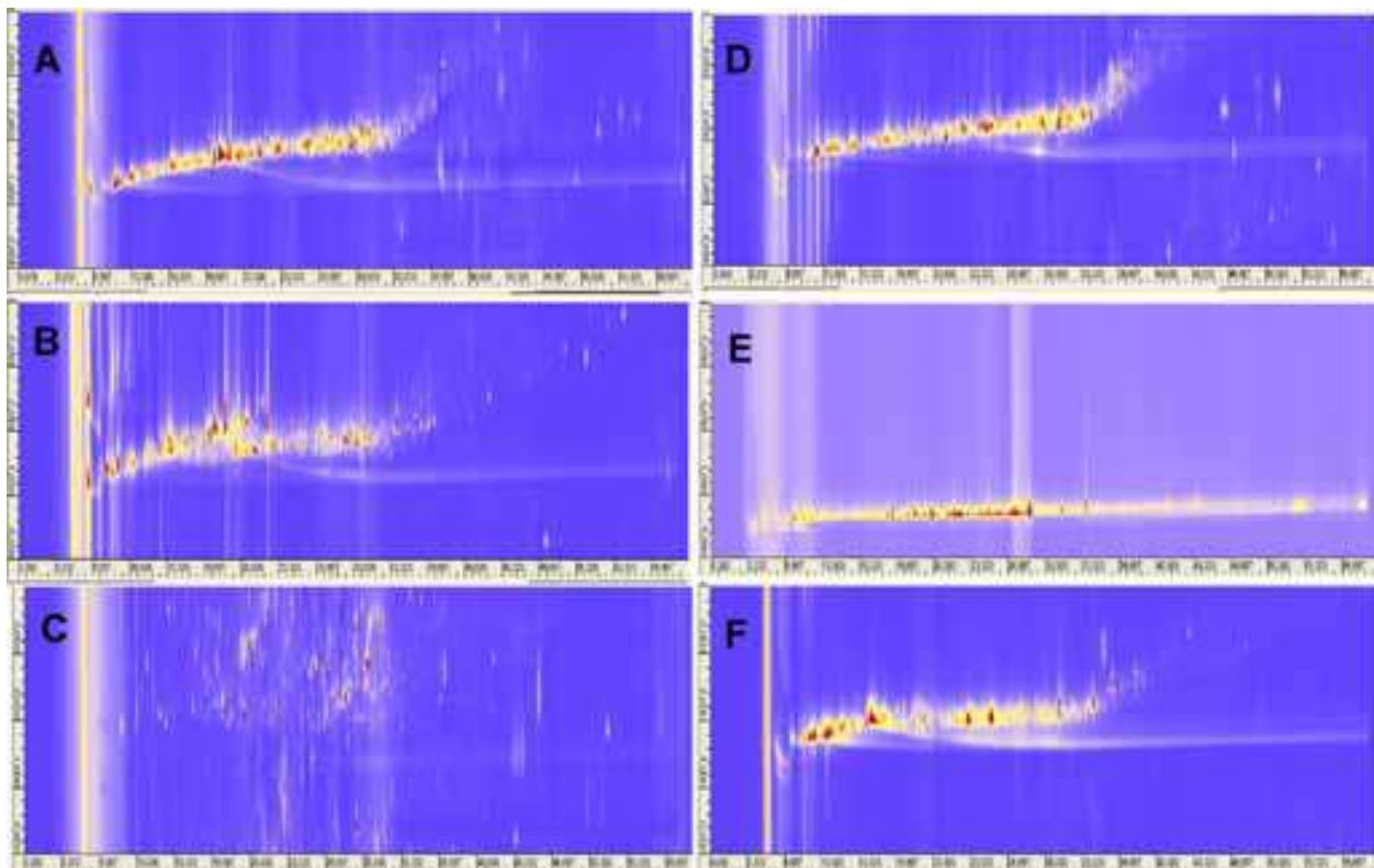
Fig. 15. Analysis of a non-spiked orange extract by GC×GC- \mu ECD using (A) ZB-5×HT-8, (B) ZB-5×BPX-50, (C) ZB-5×SW10, (D) DB-17×HT-8, (E) DB-17×BPX-50 and (F) HT-8×BPX-50 as column combinations. (From Ramos et al., 2009. With permission.).
