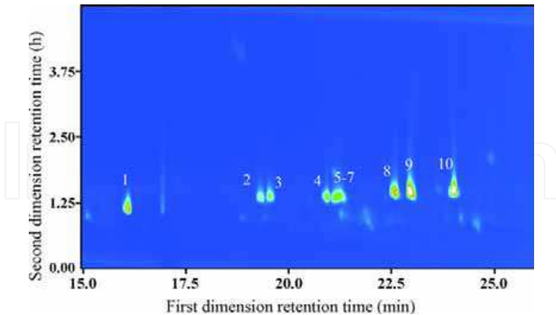
Fig. 14. GC×GC- \mu ECD contour plots for a matrix extract spiked at 0.05\text{mgkg}^{-1} with pyrethroid pesticides. Target compounds are numbered as follows: (1) bifenthrin; (2) cis -permethrin; (3) trans -permethrin; (4–7) cypermethrin (I, II, III, IV); (8) fenvalerate; (9) esfenvalerate; (10) deltamethrin. (From Pizzuti et al., 2009. With permission.).
