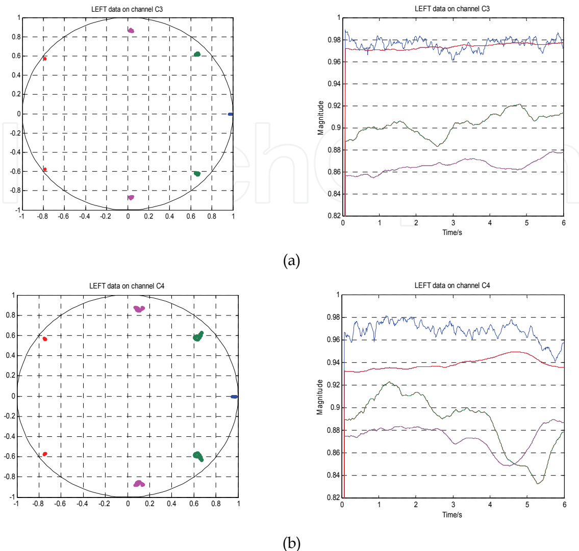
Fig. 3. Pole trajectories and magnitudes for imagined left-hand movement arising from arbitrary initialization. (a) corresponds to C3 and (b) corresponds to C4
