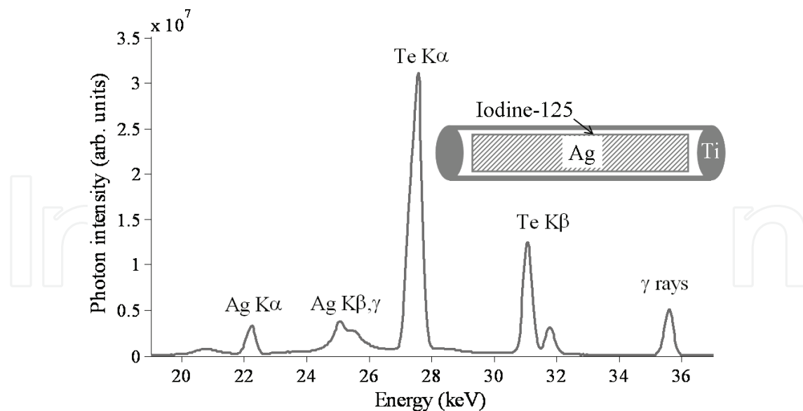
Fig. 7. Photon emission spectrum of the Amersham Health model 6711 ^{125}\text{I} seed as measured in perpendicular geometry. Gamma photons (35.49 keV) produced during ^{125}\text{I}/^{125}\text{Te} -decay as well as the most intense \text{K}\alpha and \text{K}\beta X-rays of Te are observed.
