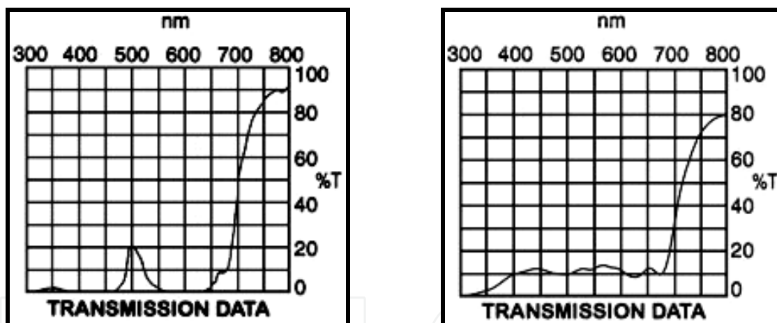
Fig. 15. CDMS – Transmission spectra of used optical filters
