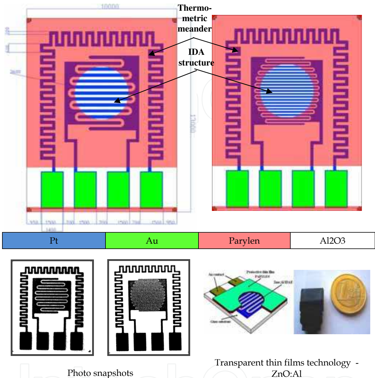
Fig. 1. IDAT microelectrodes
