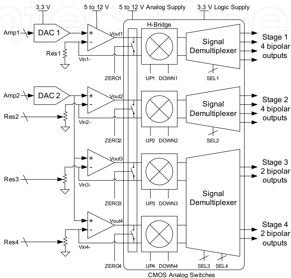
Fig. 4. Stimulation stages in UroStim8
