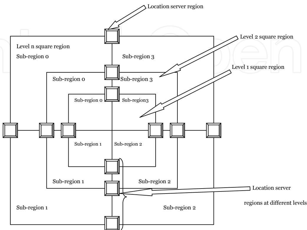
Fig. 4. Complete network structure of proposed LSLM
