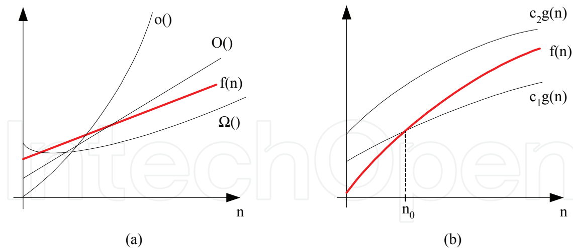
Fig. 1. (a) Interpretation of O() , o() and \Omega() ; (b) Interpretation of f(n) = \Theta(g(n)) .
