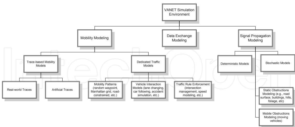
Fig. 1. Structure of VANET simulation environment
