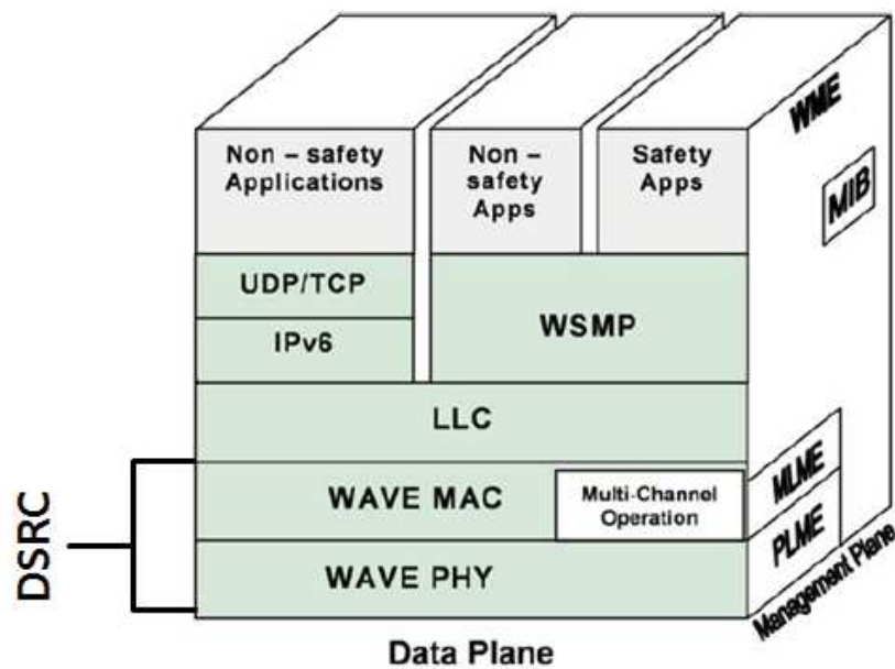
Fig. 2. WAVE protocol stack.
