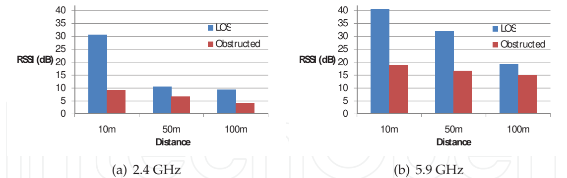
Fig. 4. RSSI measurements: average RSSI with and without the obstructing vehicle. © [2011] IEEE
