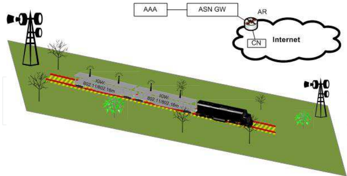
Fig. 9. SWiFT architecture
