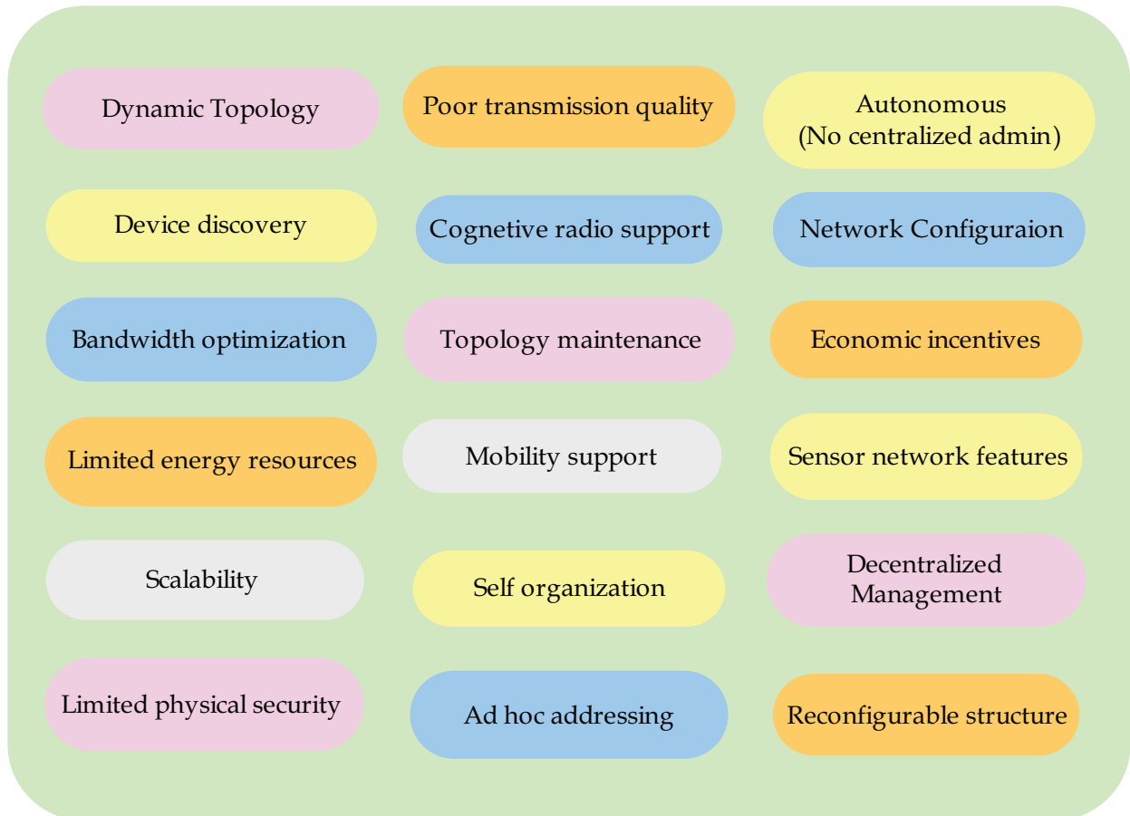
Fig. 10. Some major open issues in MANETs.
