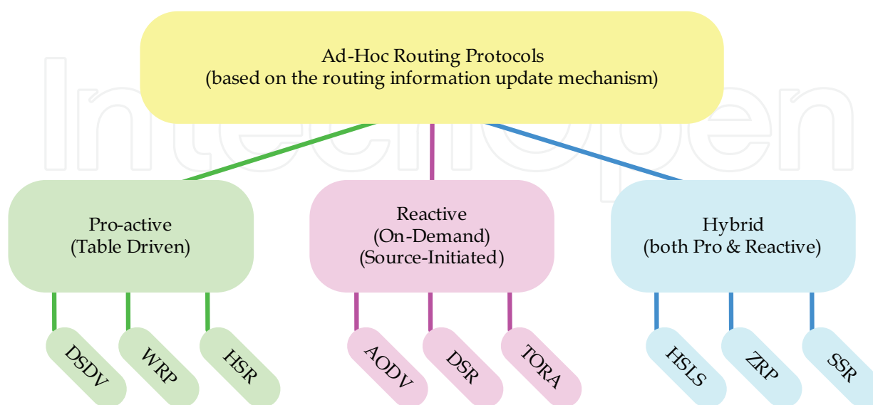
Fig. 9. Some ad-hoc routing protocols (based on the routing information update mechanism)
