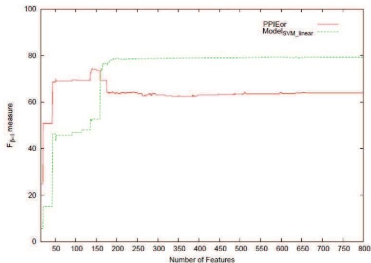
Fig. 2. Contributions of the SVM Recursive Feature Elimination (SVM RFE) algorithm to the performances of both PPIEor and Model_{SVM\_linear} . Note that x -axis is restricted to the range from 0 to 800 features since the performances do not change anymore when more features are added. The SVM RFE algorithm ranks the total of 3,543 features in a descending order according to their weights. The F_{\beta=1} measure of PPIEor with all the features is 65.58 \pm 1.31 . When the optimal parameter values obtained by 5-fold cross validation on the training data are used, PPIEor achieves the F_{\beta=1} measure of 74.10 \pm 2.11 when the top 143 features (4.04%) are used. For Model_{SVM\_linear} , the best F_{\beta=1} measure of 79.35 is obtained when the top 635 features are used while the F_{\beta=1} measure for all the features is 79.17.
