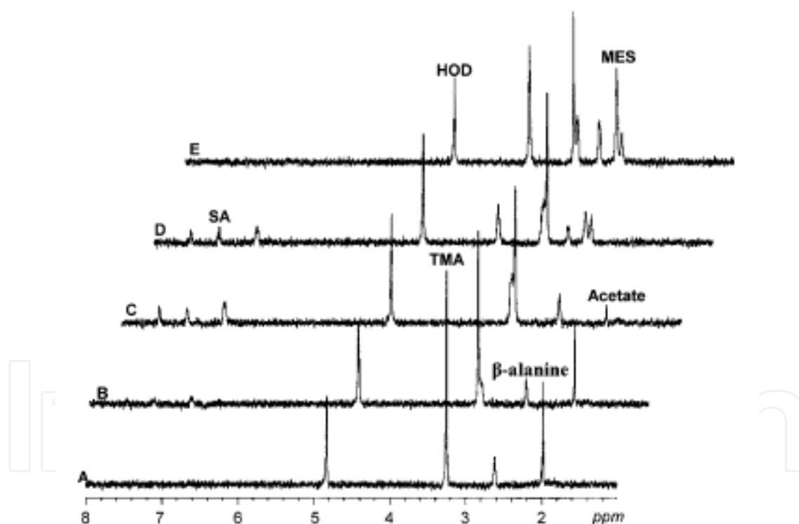
Fig. 1. Profile of the migration of ions in the course of an anionic cITP-NMR experiment. The buffers used were 160 mM DCl/80 mM \beta -alanine/20 mM TMA acetate (LE) and 160 mM MES (TE). The analyte is 250 \mu M salicylate. Spectrum A contains the resonances of the LE only (TMA acetate and \beta -alanine). In spectrum B, the salicylate resonances (SA) begin to emerge in the aromatic region of the spectrum and become more intense in spectra C and D. The TE resonances (MES) begin to emerge in spectrum D, becoming more intense in E. Note that the acetate resonances are detected only up to spectrum C. Reprinted with permission from Analytical Chemistry , 2006, 78, 7078-7087. Copyright 2006 American Chemical Society.
