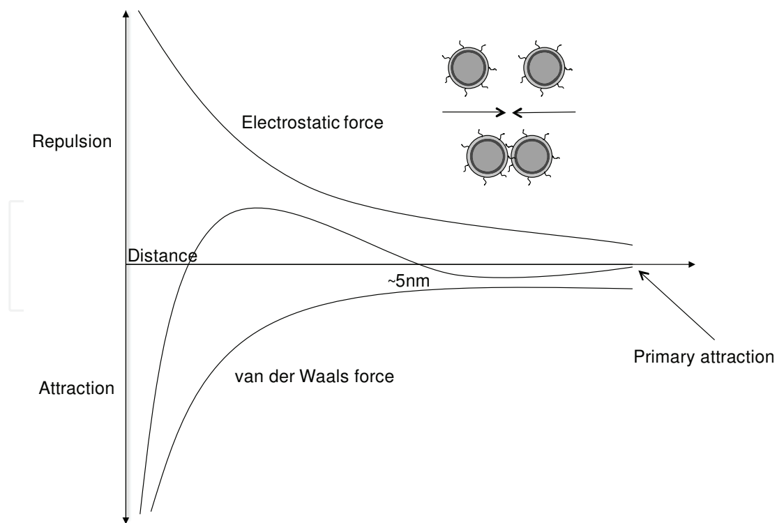
Fig. 2. The DLVO theory
