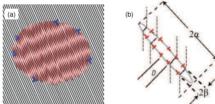
Fig. 18. (a) Schematic illustrating (a) rotation of a local volume through stacked dislocation loops (Cui et al., 2009), and (b) the incipient kink band mechanism (Barsoum et al., 2003).
