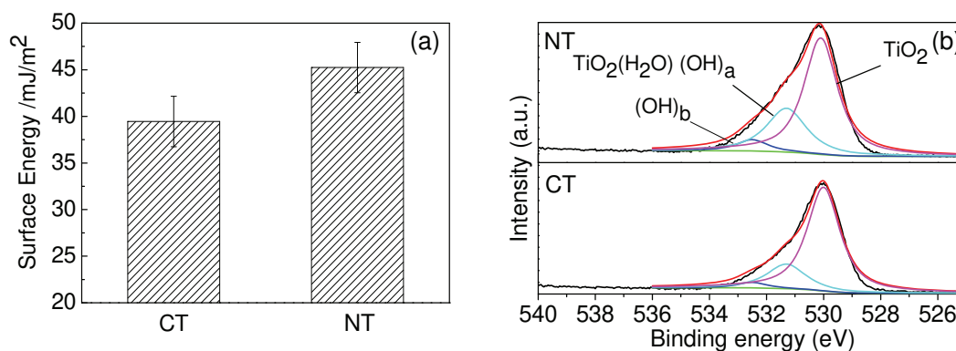
Fig. 24. (a) Comparison of surface energy of CT and NT samples; (b) x-ray photoelectron spectrum O 1s peaks obtained from CT and NT samples (Zheng, 2009).
