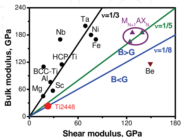
Fig. 14. A collection of shear and bulk moduli of some metals and metal-like ceramics M_{N+1}AX_N in comparison with Ti2448 (Hao, Li, Sun, Sui & Yang, 2007).
