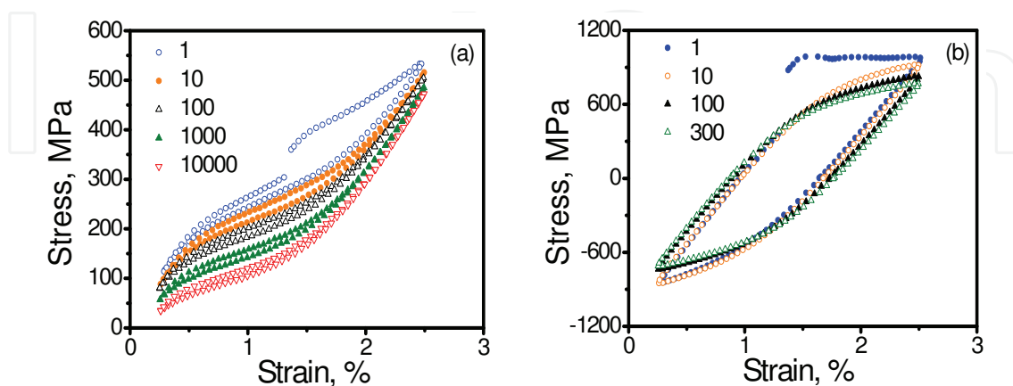
Fig. 11. Hysteresis loop of as-forged Ti–24Nb–4Zr–7.6Sn (a) and Ti–6Al–4V ELI (b) recorded at different cycles of maximum strain 2.5% during the low cycle fatigue test (Li, Cui, Hao & Yang, 2008).
