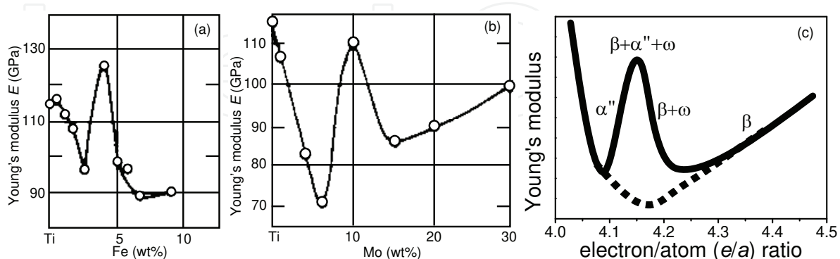
Fig. 1. Young's moduli, E , of Ti-Fe (a) and Ti-Mo (b) alloys as functions of composition (Fedotov, 1973). A schematic of the E vs. e/a plot for Ti-TM alloys is shown in (c) with the dotted curve indicating the intrinsic minimum in E of the \beta phase (Hao, Li, Sun, Zheng & Yang, 2007).
