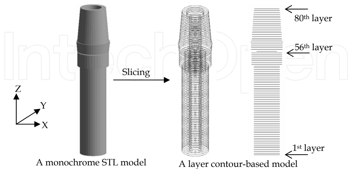
Fig. 18. Slicing an STL model of a dental implant assembly into a contour-based model for FGM modelling
