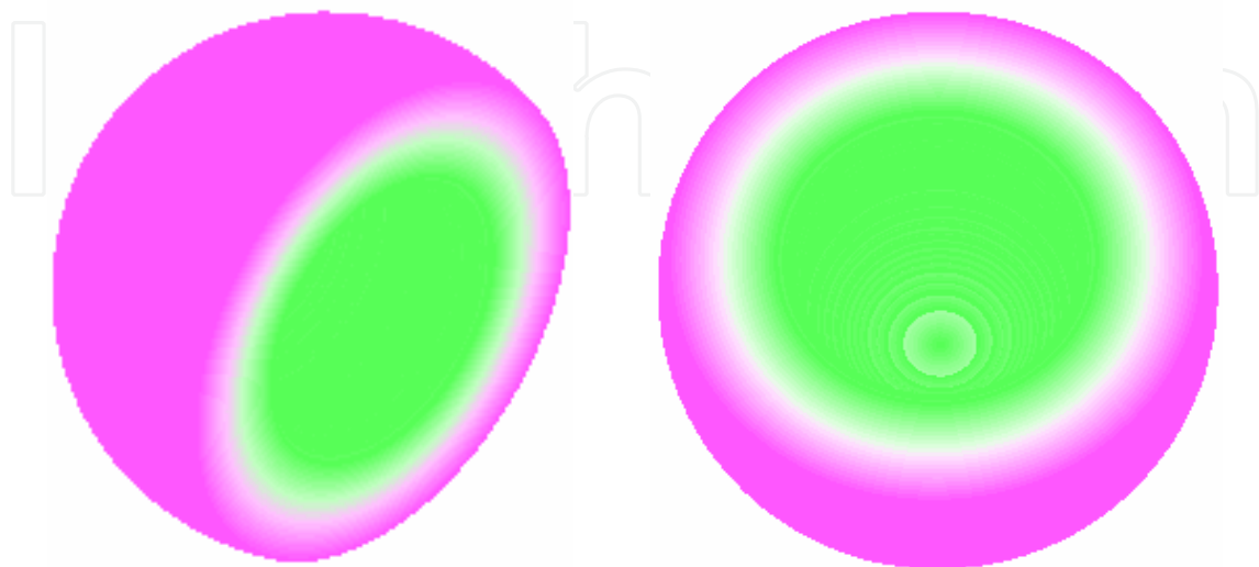
Fig. 14. A contour-based FGM model of the acetabular cup from two perspectives
