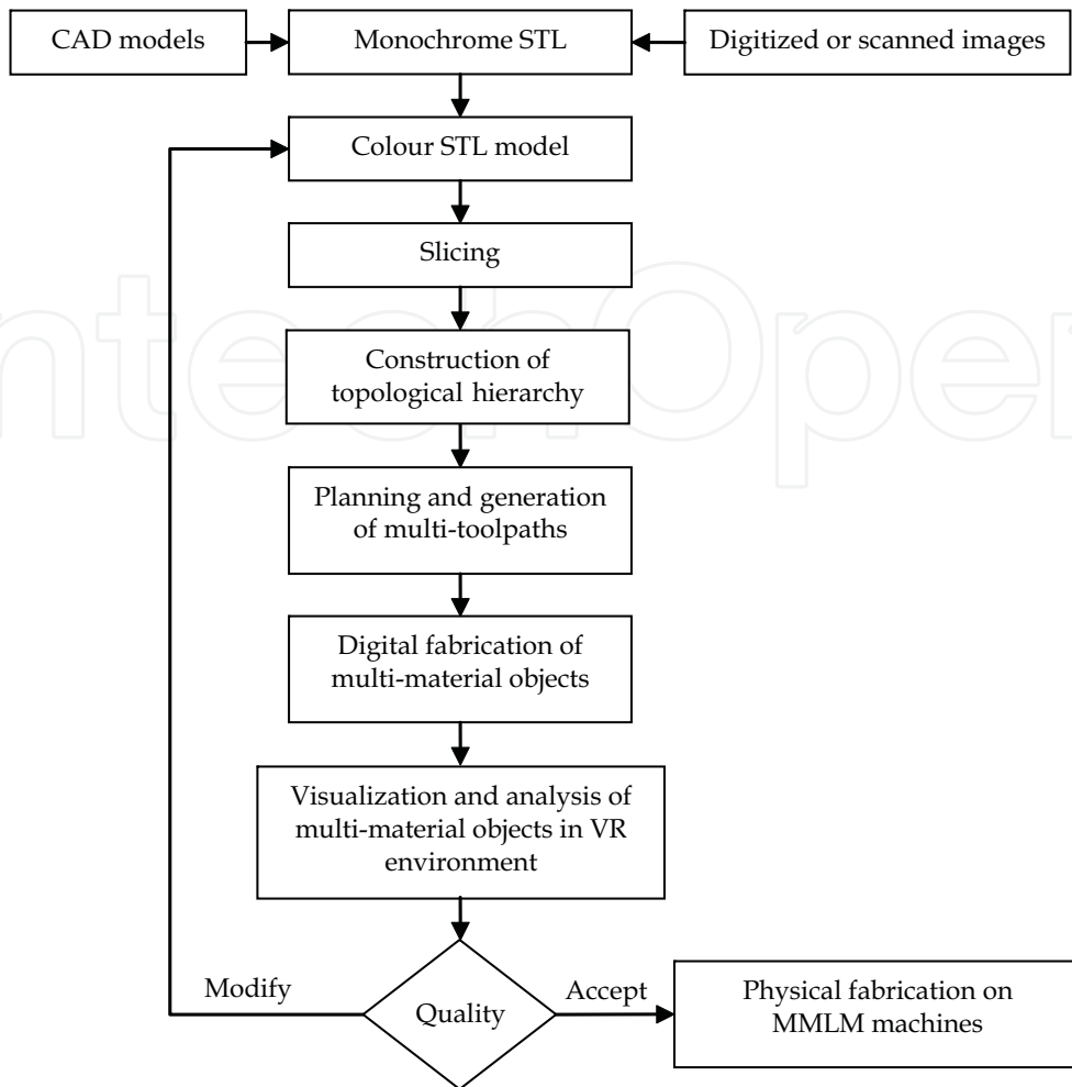
Fig. 1. The flow of the DMMVP module
