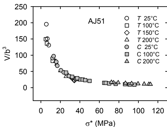
Fig. 11. Plot of the apparent activation volume (in b^3 ) against the thermal stress \sigma^* estimated for four deformation temperatures in tension (T) and compression (C) for the AJ51 alloy.
