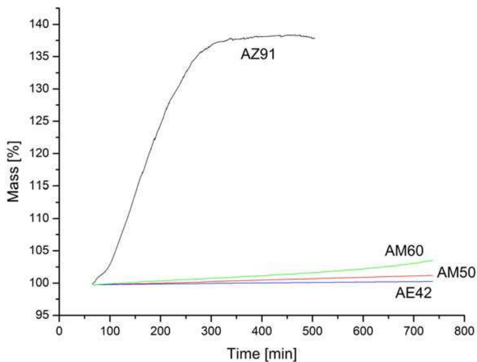
Fig. 9. Mass changes as function of time for all samples at 450 °C
