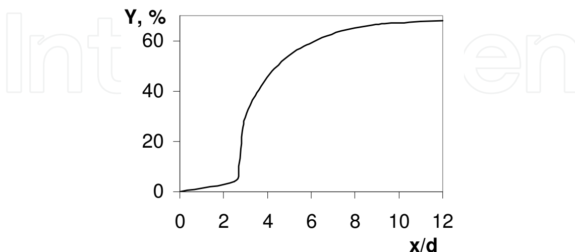
Fig. 4. Dependence of melting degree of 50 \mu\text{m Al}_2\text{O}_3 particle from spraying distance
