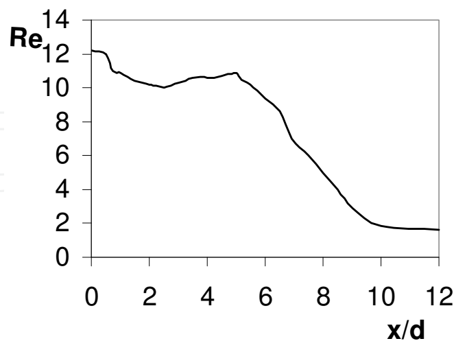
Fig. 3. Variation of Reynolds number along spraying distance
